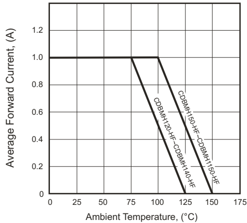
Fig.1- Typical Current Derating Curve
