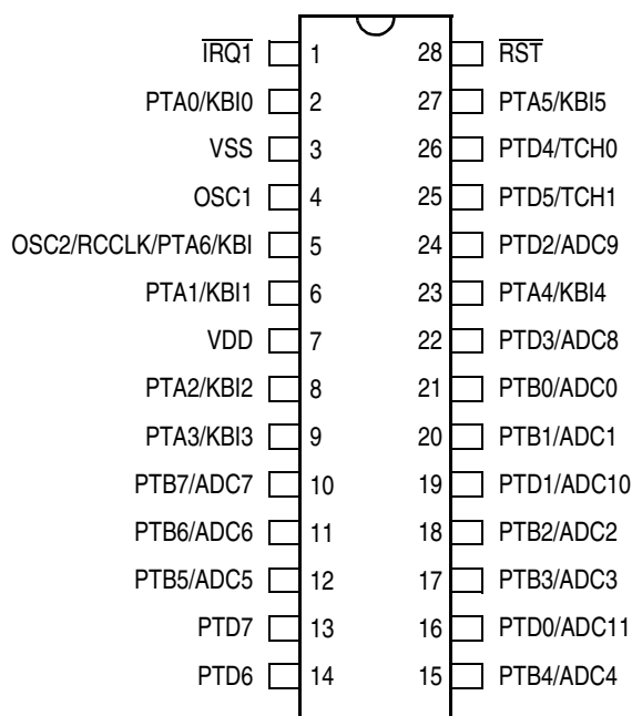
MC68H(R)C908JL3E
