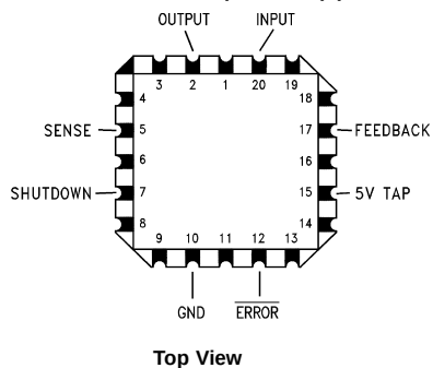
Leadless Chip Carrier (E)
