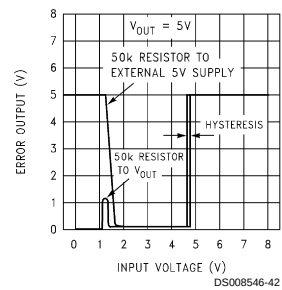
LP2951 Error Comparator Output
