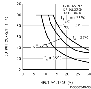
LP2951 Maximum Rated Output Current
