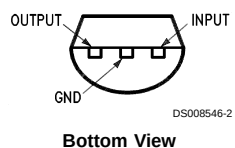
TO-92 Plastic Package (Z)
