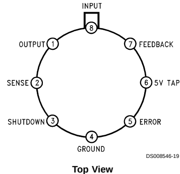
Metal Can Package (H)
