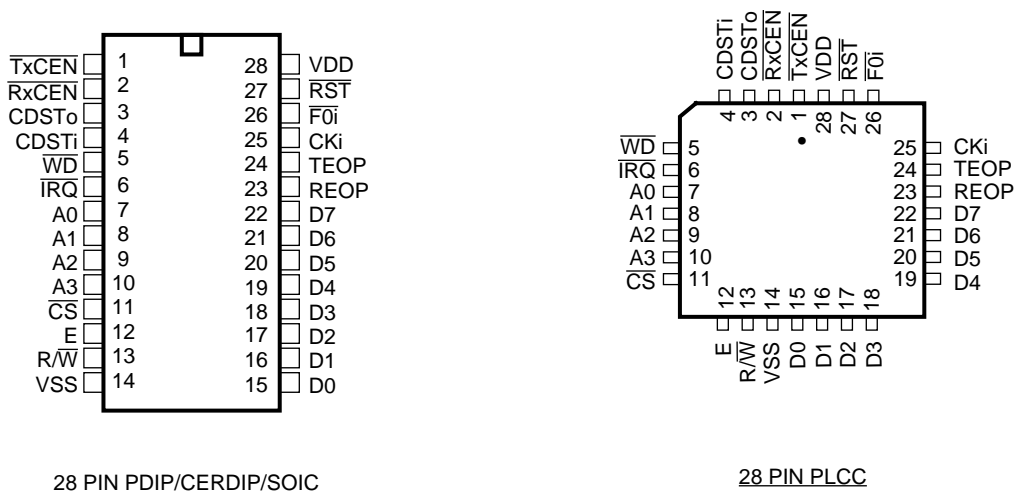
Figure 2 - Pin Connections
