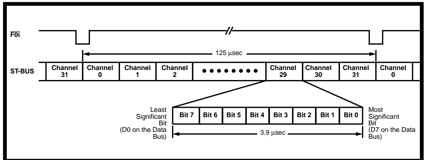
Figure 24 - ST-BUS Format
