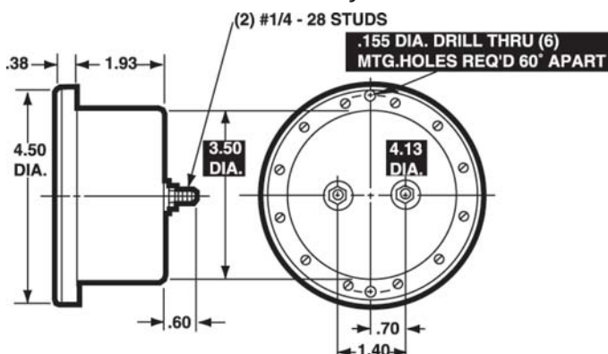
4 - 1/2"-Model 2524, 2544 Round Style
