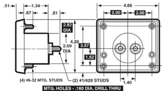
4-1/2"-Model 2124, 2124T, 2144, 2154, 2184
