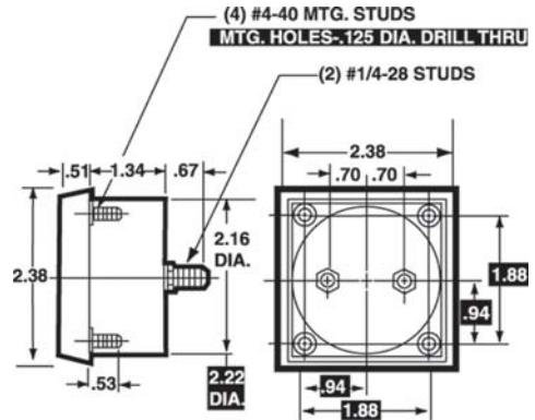
2-1/2"-Models 2122, 2122T, 2142, 2152, 2182
