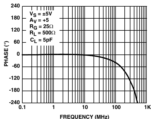
FIGURE 2. PHASE vs FREQUENCY
