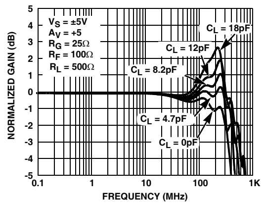
FIGURE 10. GAIN vs FREQUENCY FOR VARIOUS C_{LOAD} ( A_V = +5 )
