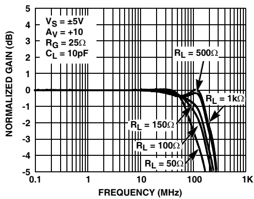
FIGURE 9. GAIN vs FREQUENCY FOR VARIOUS R_{LOAD} ( A_V = +10 )
