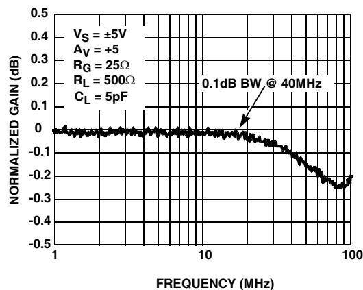
FIGURE 3. 0.1dB BANDWIDTH
