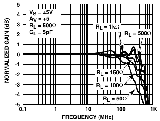
FIGURE 8. GAIN vs FREQUENCY FOR VARIOUS R_{LOAD}
