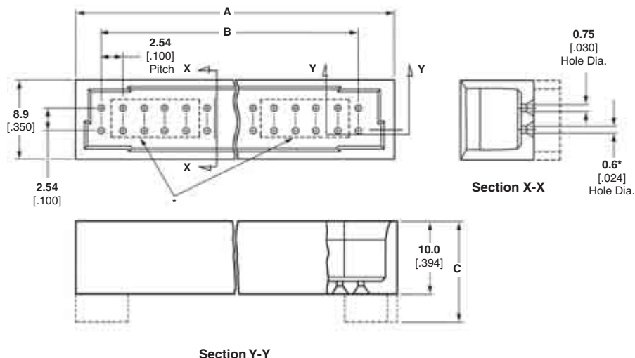
Section Y-Y
