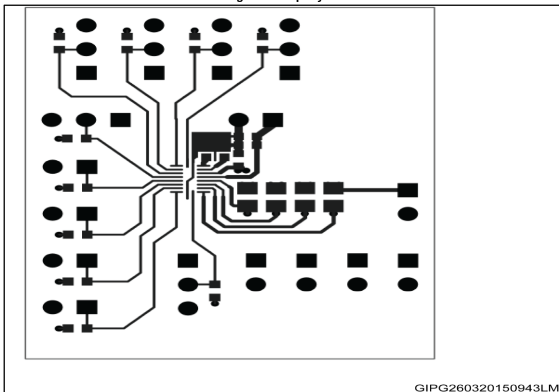
Figure 9: Top layer
