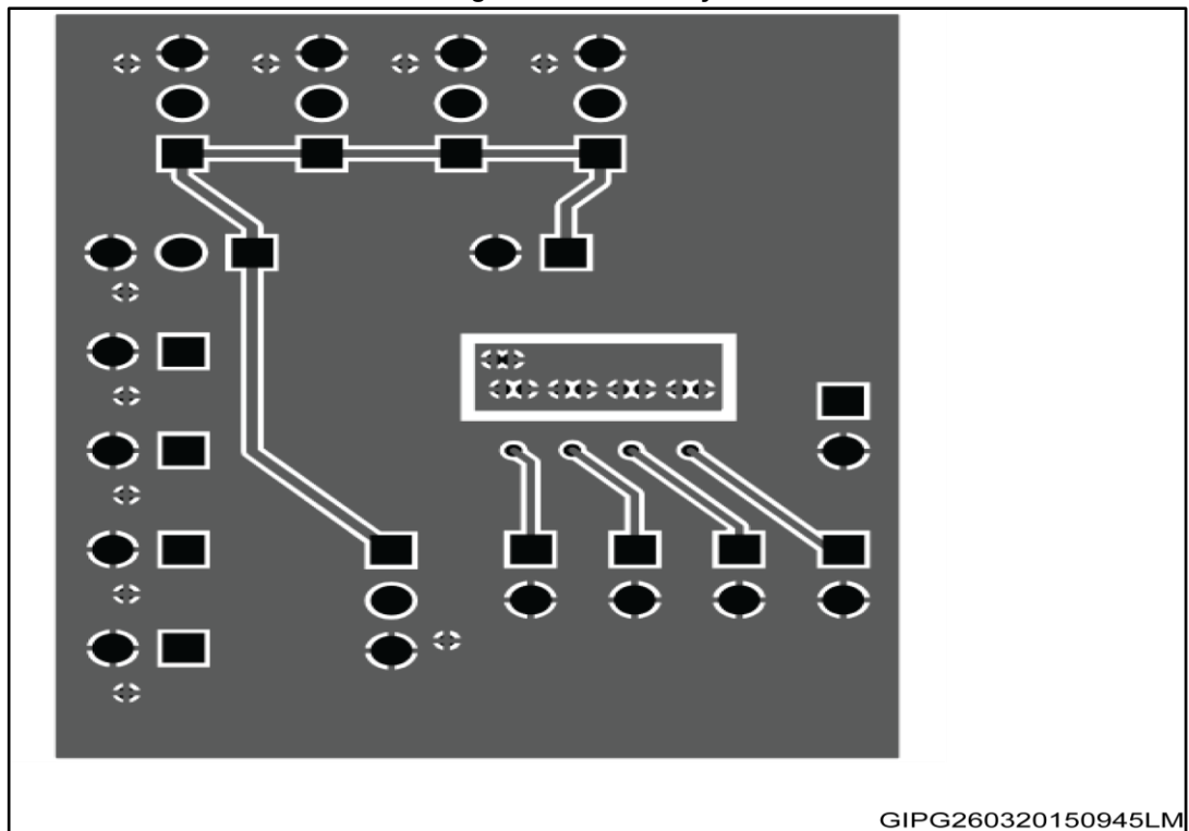
Figure 11: Top overlay
