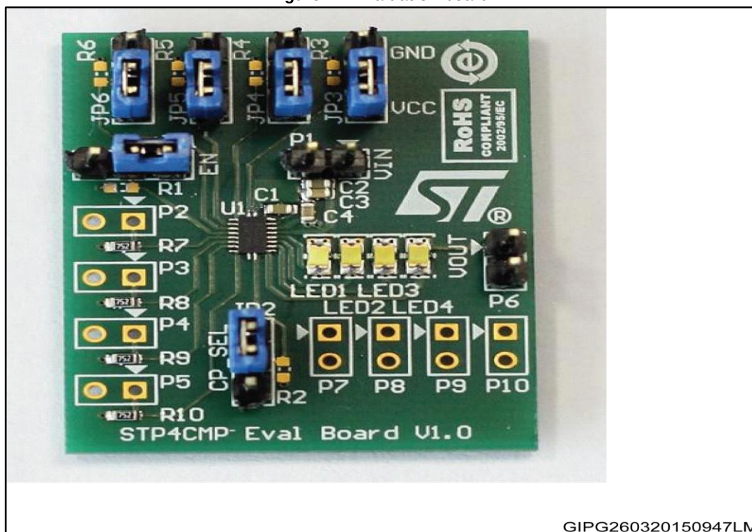
Figure 12: Evaluation board
