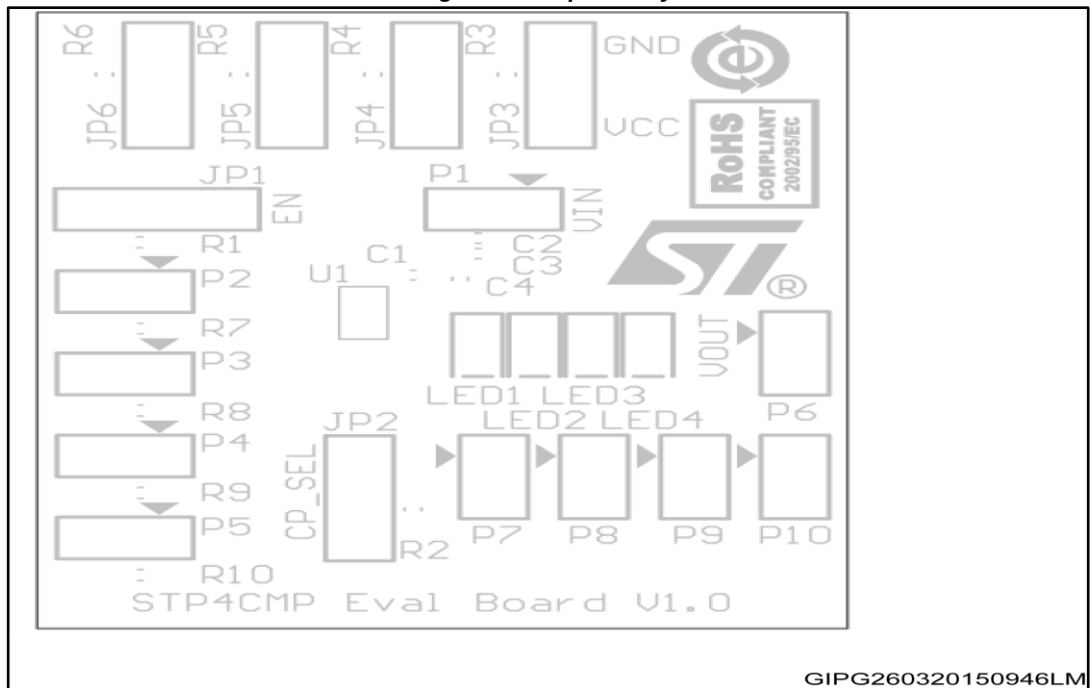
Figure 11: Top overlay
