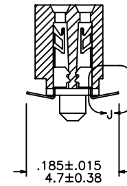
SECTION X-X
