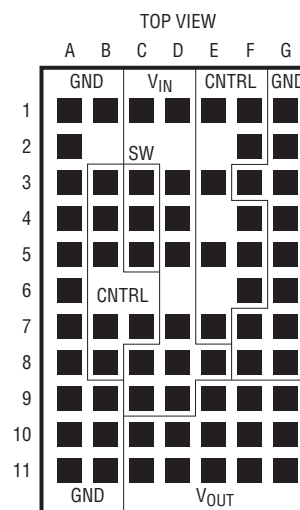
LGA PACKAGE 68-LEAD (15mm × 9mm × 2.82mm)
