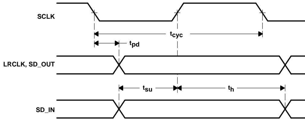
Figure 3–6. I 2 S Mode Timing Waveforms
