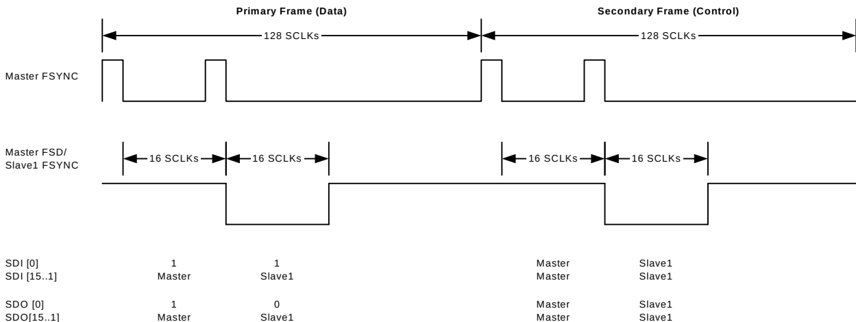
Figure 32. Daisy Chaining of a Single Slave (Frame FSD)
