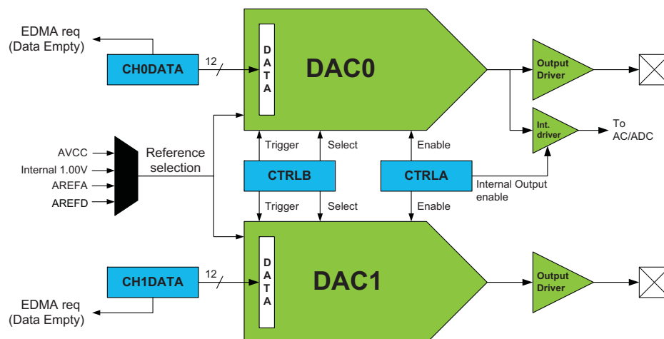
Figure 29-1. DAC overview.
