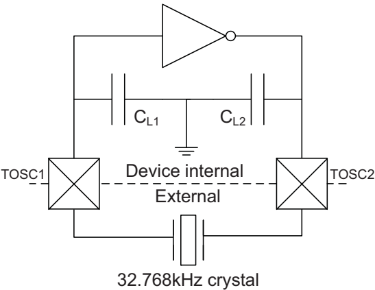
Figure 36-4. TOSC input capacitance.
