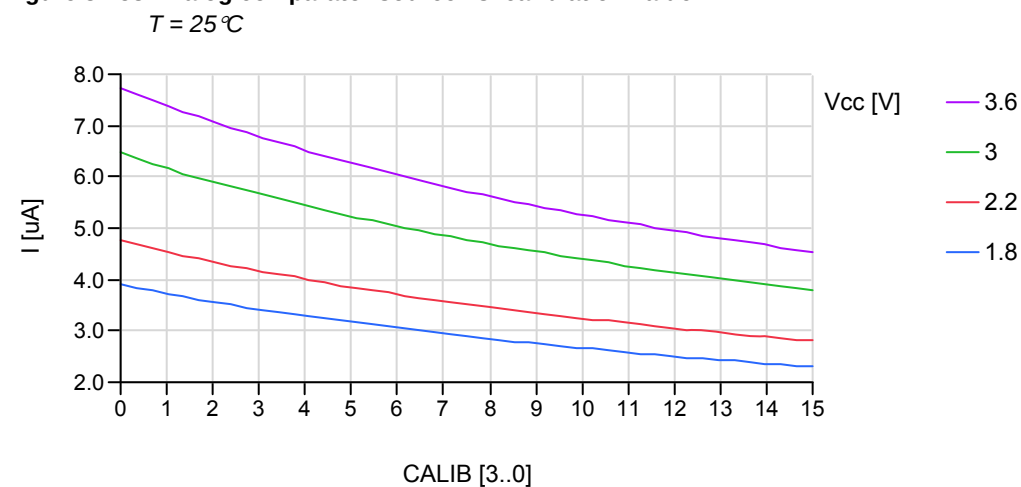
Figure 37-58. Analog comparator source vs. calibration value.
