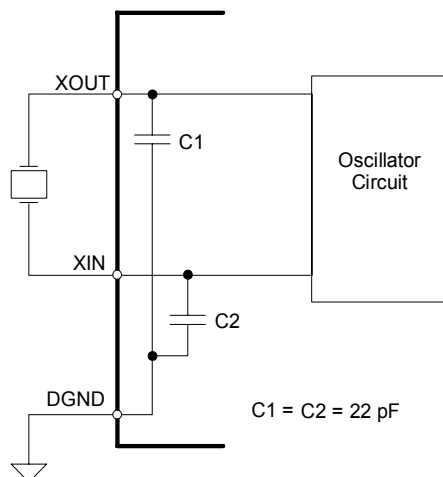
Figure 3. Oscillator Connection
