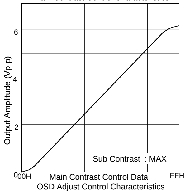
Main Contrast Control Characteristics
