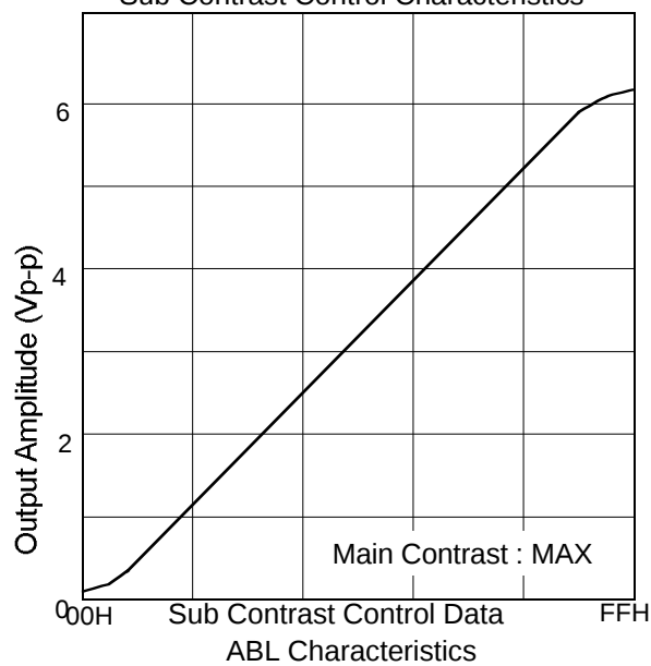
Sub Contrast Control Characteristics
