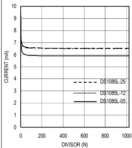
SUPPLY CURRENT vs. DIVISOR
