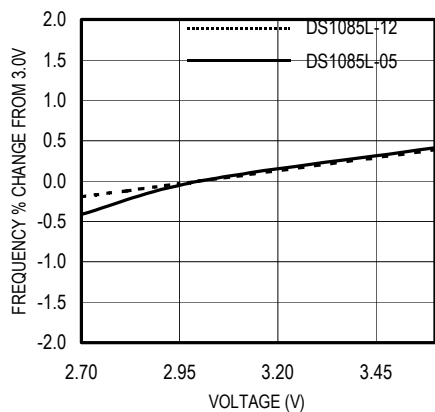
FREQUENCY % CHANGE vs. SUPPLY VOLTAGE
