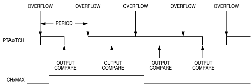
Figure 15-9. CHxMAX Latency
