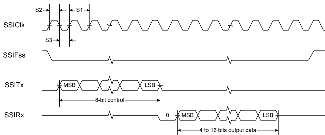
Figure 18-12. SSI Timing for MICROWIRE Frame Format (FRF=10), Single Transfer
