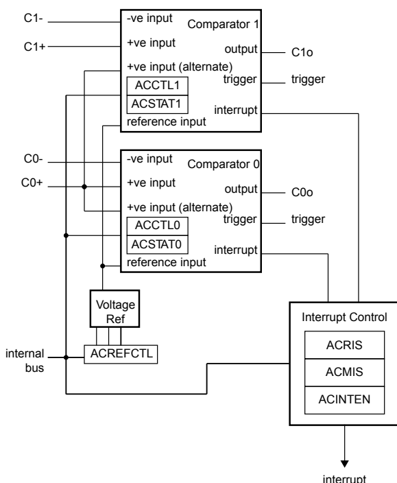
Figure 14-1. Analog Comparator Module Block Diagram
