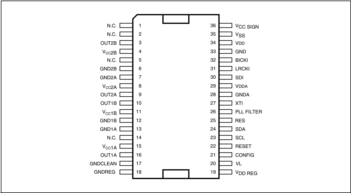
Figure 9. Pin Description
