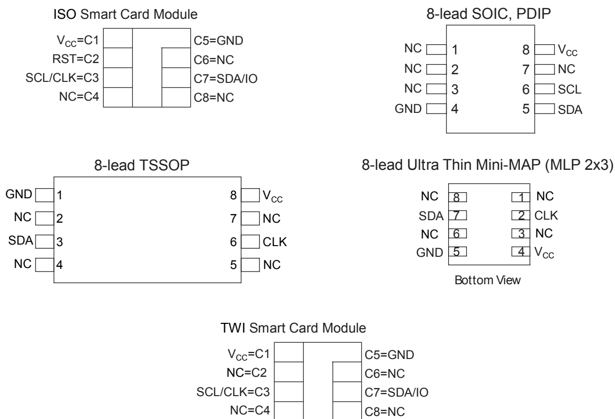
Figure 1. Pin Configuration
