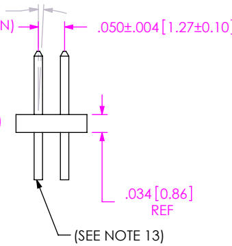
FIG 1 FTS-1XX-01-XX-D SHOWN
