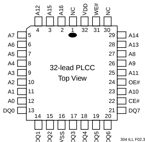
FIGURE 1: PIN ASSIGNMENTS FOR 32-LEAD PLCC
