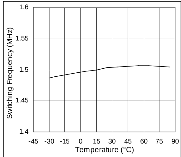
Figure 10. Switching Frequency vs. Temperature
