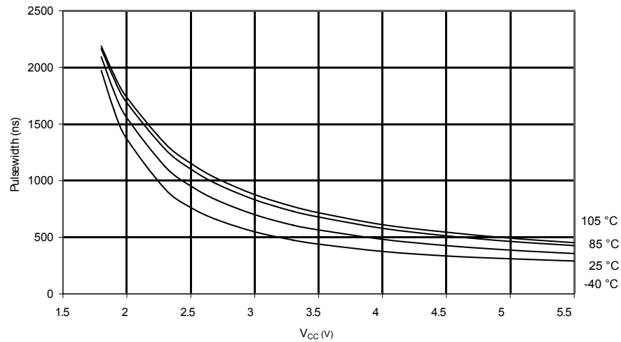
Figure 30-47. Minimum Reset Pulswidth vs. V_{CC}
