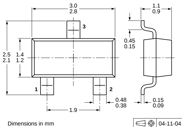
Fig 14. Package outline PDTTC114YT (SOT23)
