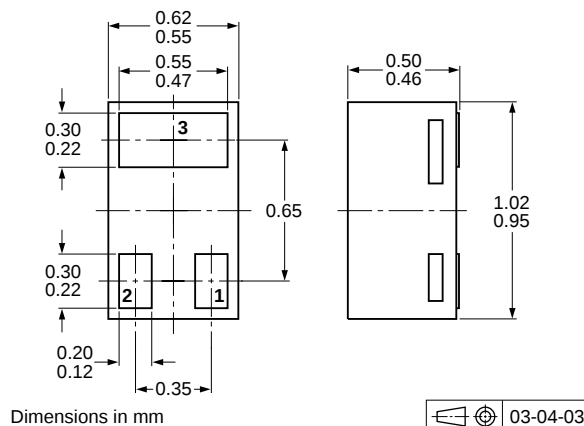
Fig 13. Package outline PDTTC114YM (SOT883/SC-101)
