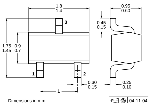
Fig 12. Package outline PDTTC114YE (SOT416/SC-75)
