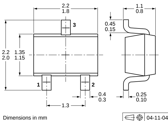
Fig 15. Package outline PDTTC114YU (SOT323/SC-70)
