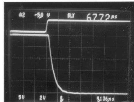
Figure 3. Settling time
