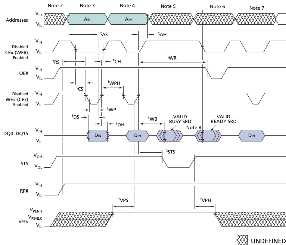
Figure 20: WRITE Operations
