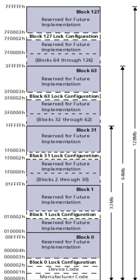
Figure 7: Device Identifier Code Memory Map
