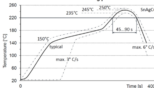
Resistance to soldering heat
