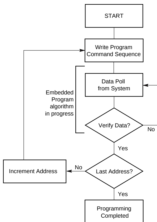
Figure 2. Program Operation
