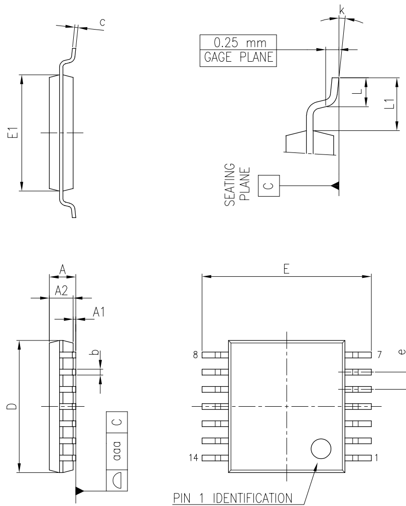
Figure 27. TSSOP-14 package outline
