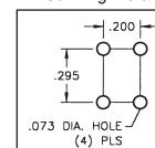
PC MOUNT
