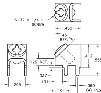
PC MOUNT
