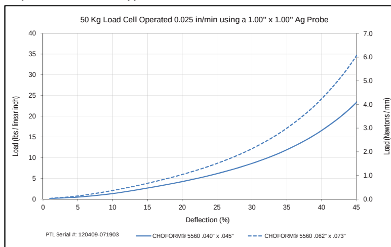
Graph 8-1 Deflection vs Applied Load
