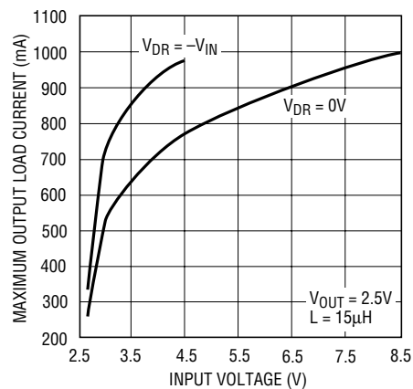
Maximum Output Load Current vs Input Voltage
