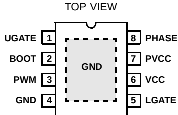
ISL6612BCB, ISL6613BCB, ISL6612BECB, ISL6613BECB (8 LD SOIC, EPSONIC)
