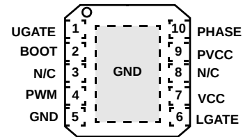
ISL6612BCR, ISL6613BCR (10 LD 3x3 DFN) TOP VIEW
