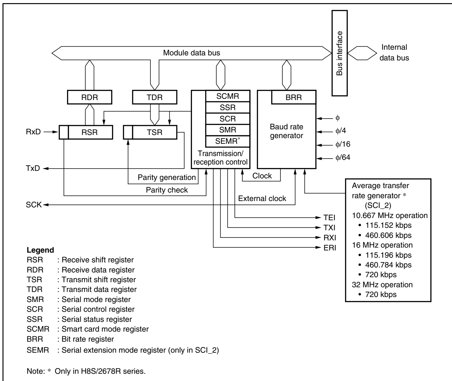
Figure 15.1 Block Diagram of SCI
