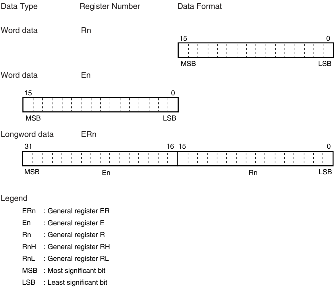
Figure 2.9 General Register Data Formats (2)
