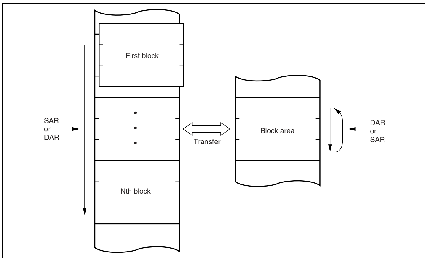
Figure 9.7 Memory Mapping in Block Transfer Mode
