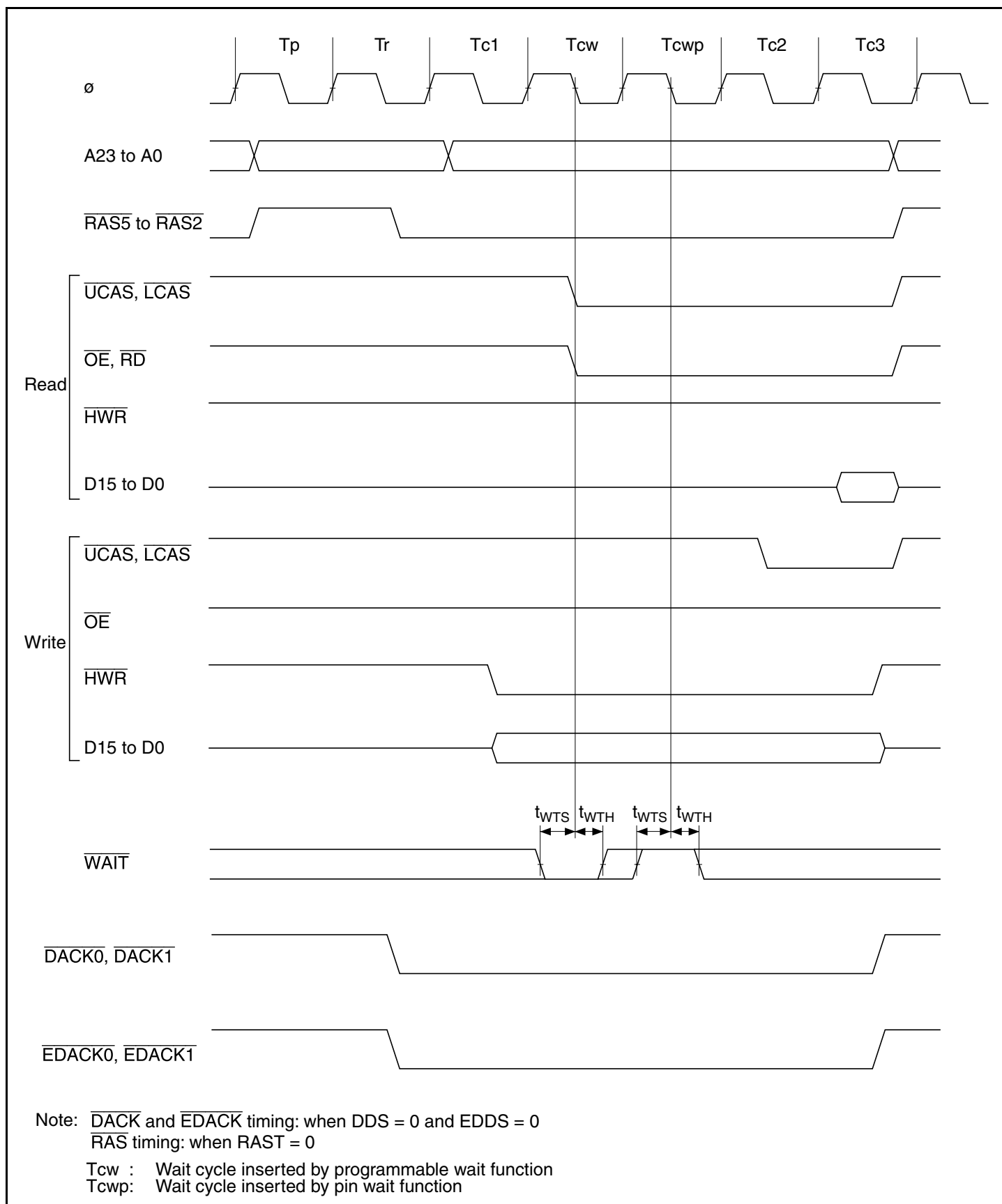
Figure 24.18 DRAM Access Timing: Three-State Access, One Wait
