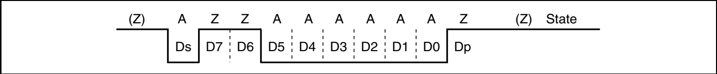
Figure 15.24 Inverse Convention (SDIR = SINV = O/E = 1)
