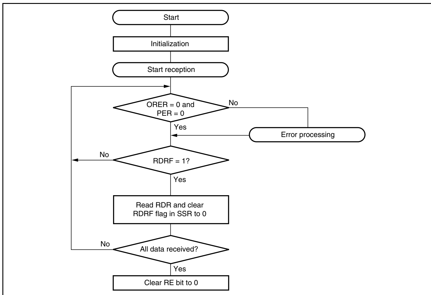
Figure 15.30 Example of Reception Processing Flow
