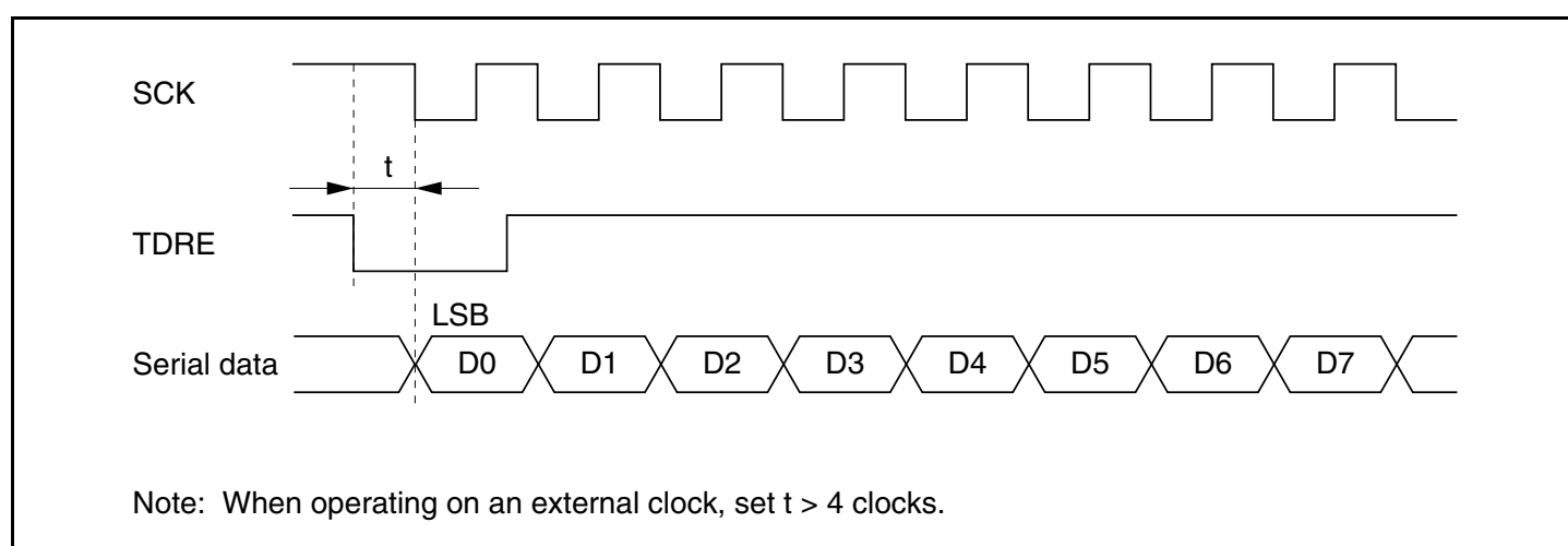
Figure 15.35 Example of Synchronous Transmission Using DTC
