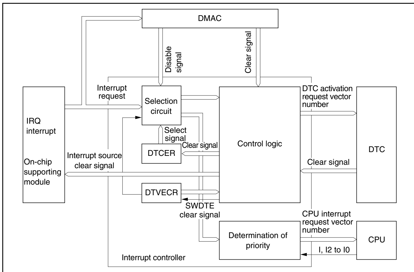
Figure 5.6 DTC, DMAC, and Interrupt Controller
