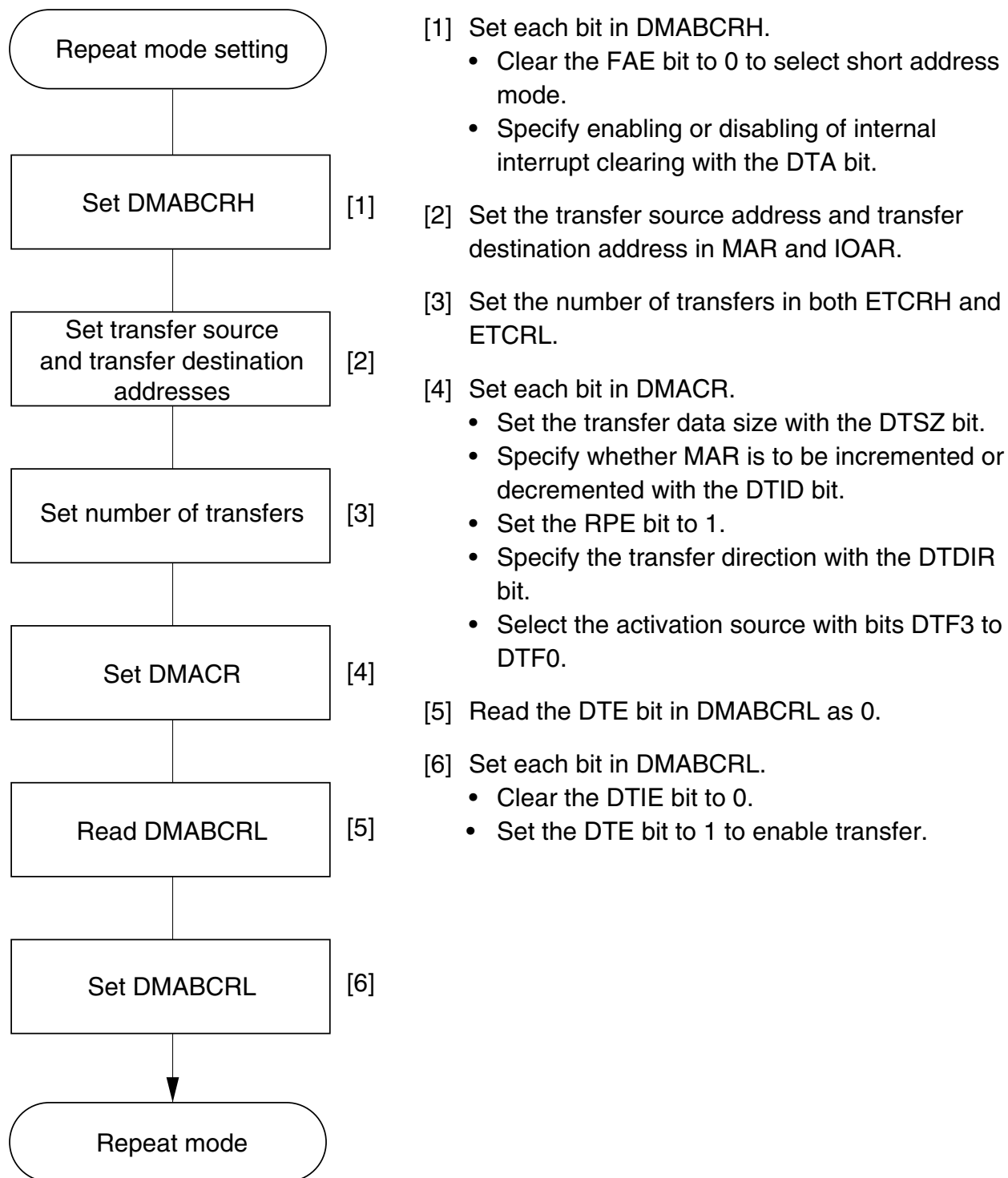
Figure 7.8 Example of Repeat Mode Setting Procedure
