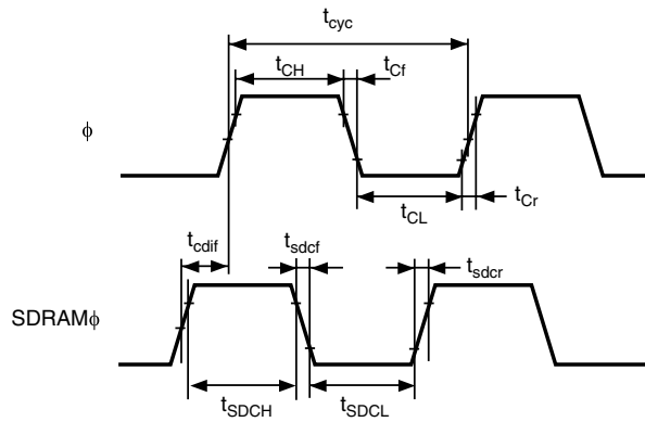
Figure 24.3 SDRAMφ Timing*
