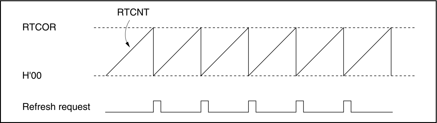
Figure 6.34 RTCNT Operation
