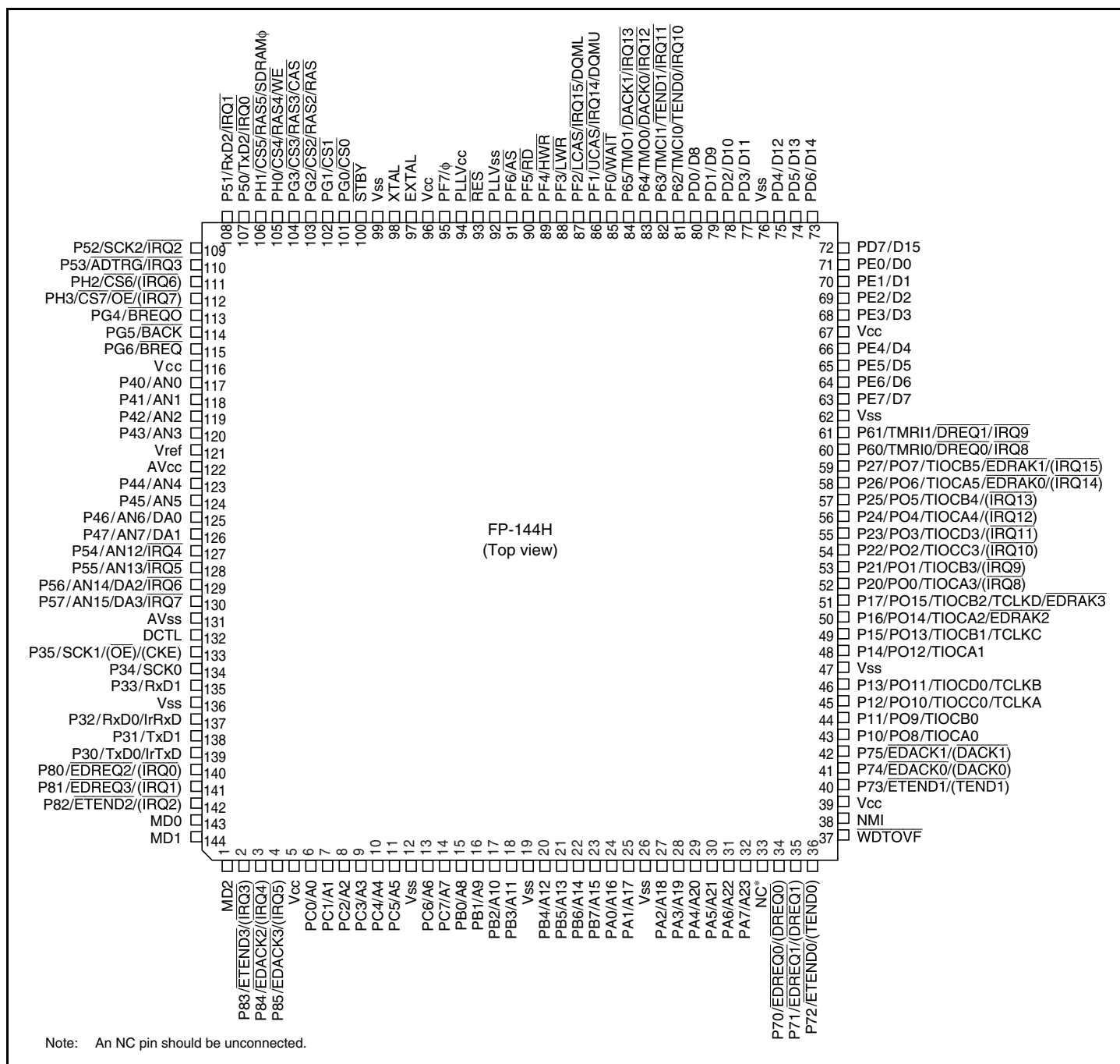
Figure 1.4 H8S/2678R Series Pin Arrangement
