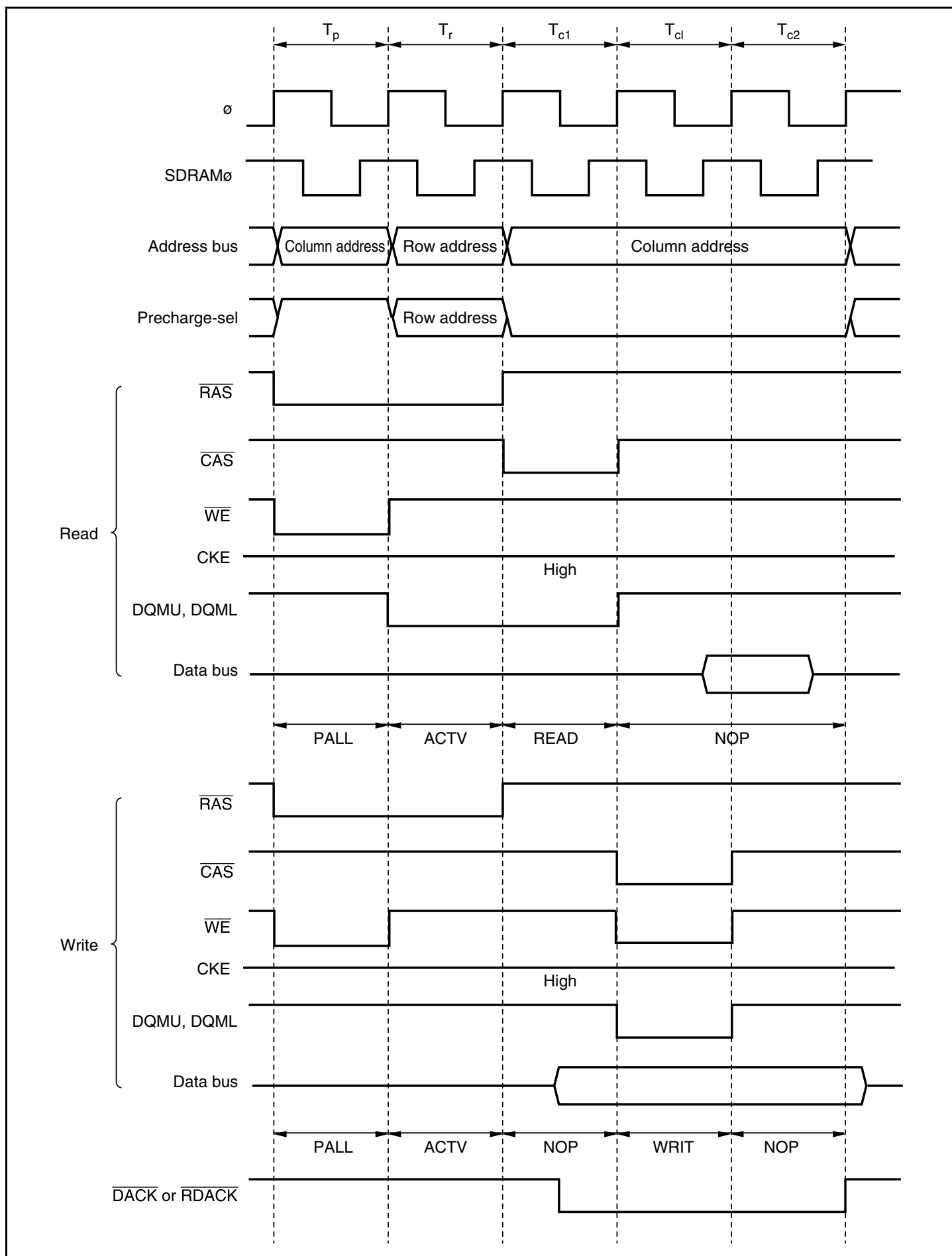
Figure 6.60 Example of DACK/EDACK Output Timing when DDS = 1 or EDDS = 1
