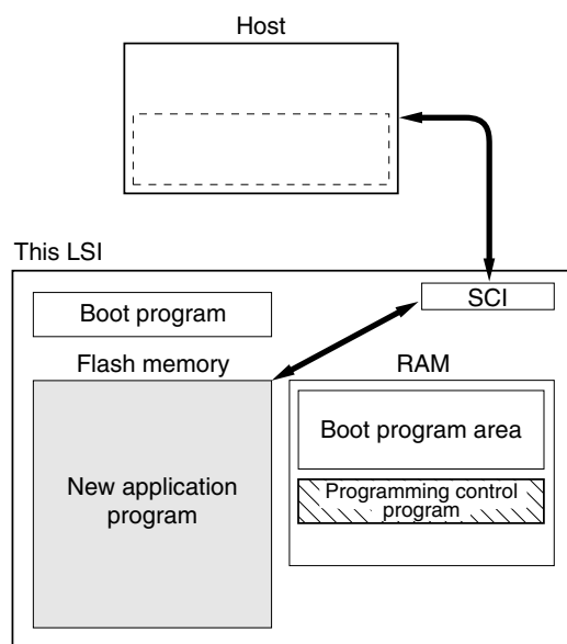
Figure 19.3 Boot Mode
