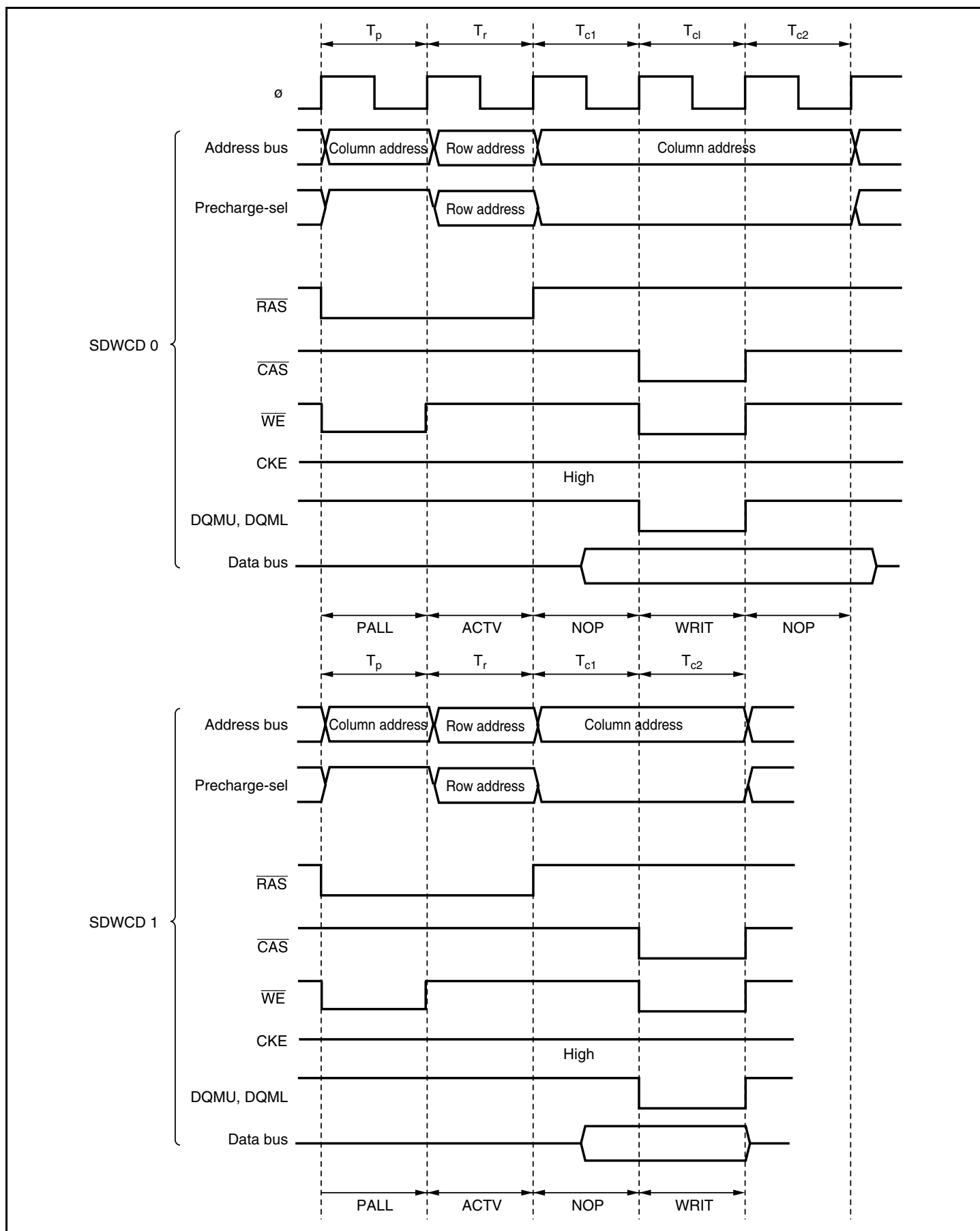
Figure 6.5 CAS Latency Control Cycle Disable Timing during Continuous Synchronous DRAM Space Write Access (for CAS Latency 2)
