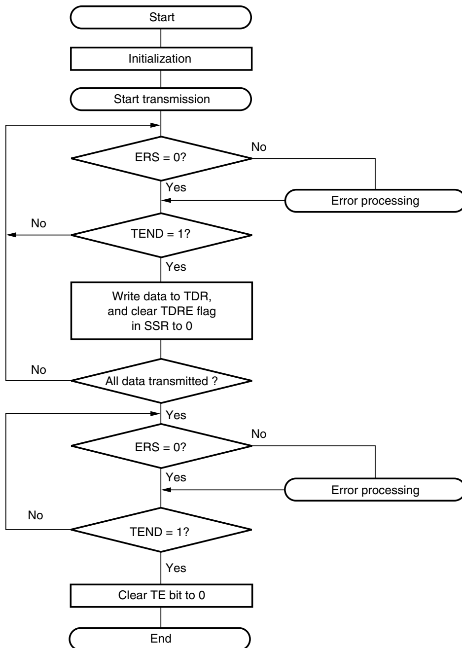
Figure 15.28 Example of Transmission Processing Flow
