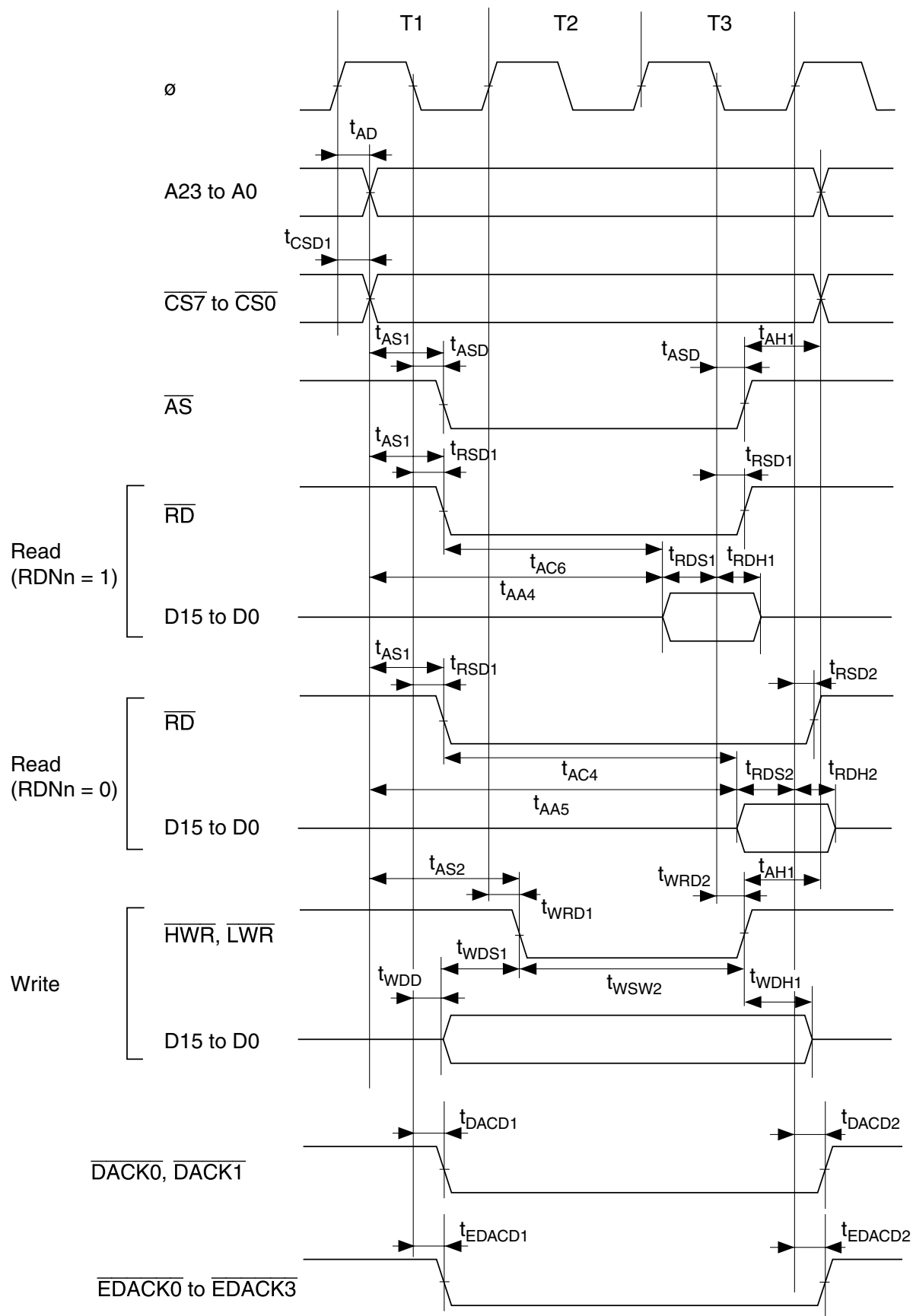
Figure 24.8 Basic Bus Timing: Three-State Access
