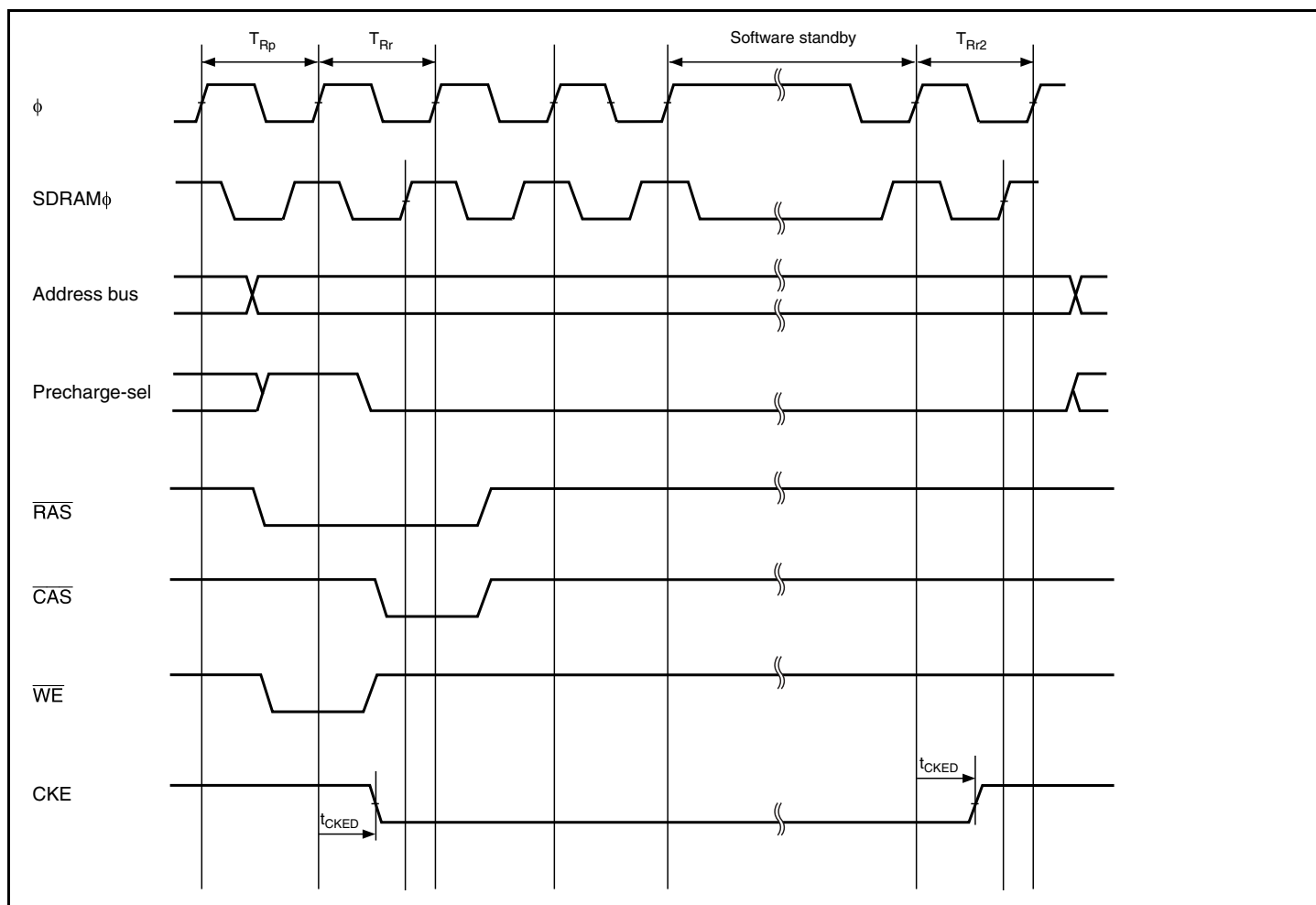
Figure 24.27 Synchronous DRAM Self-Refresh Timing
