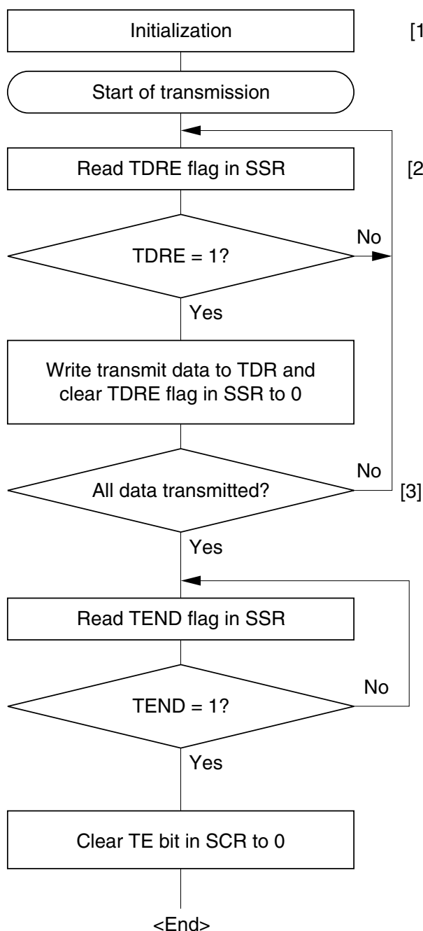
Figure 15.17 Sample Serial Transmission Flowchart
