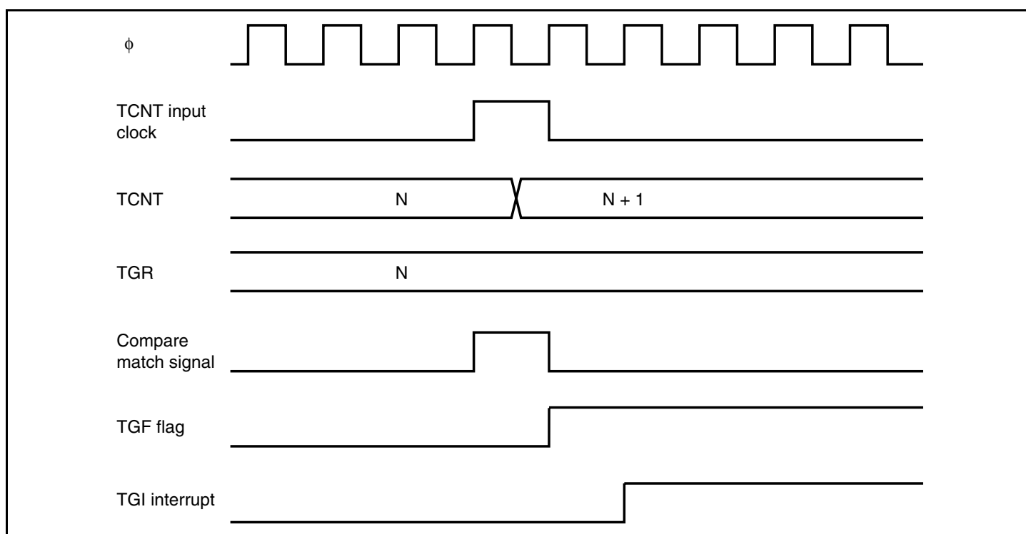
Figure 11.38 TGI Interrupt Timing (Compare Match)
