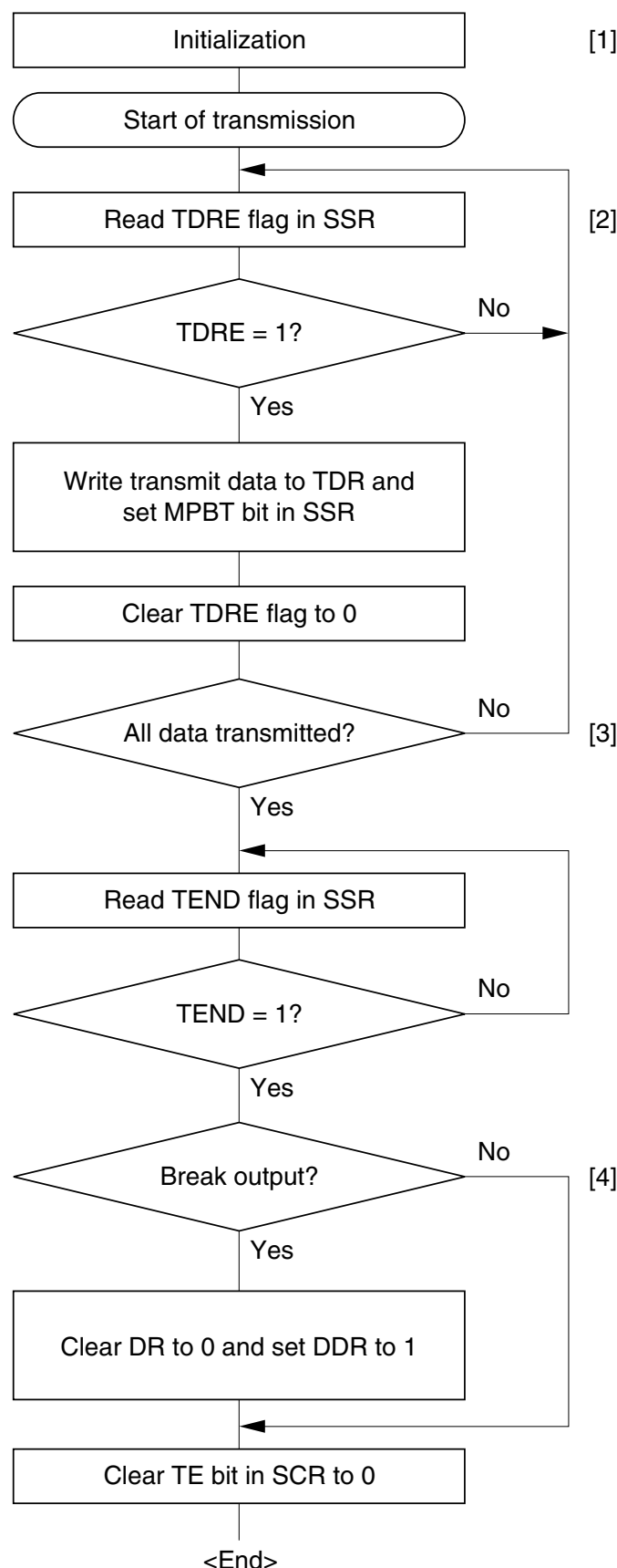
Figure 15.11 Sample Multiprocessor Serial Transmission Flowchart
