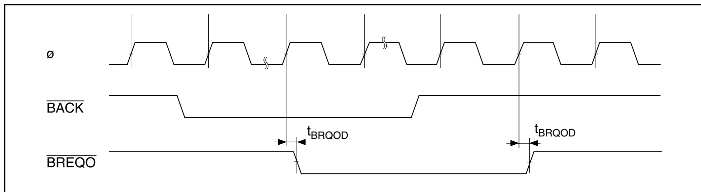
Figure 24.25 External Bus Request Output Timing
