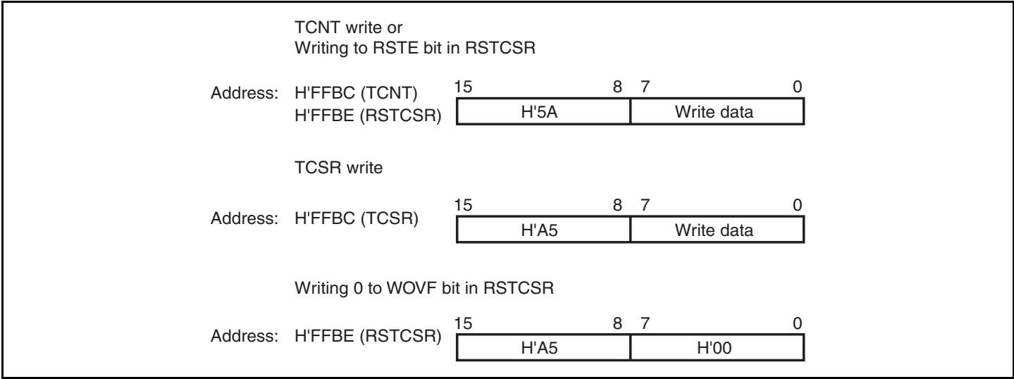
Figure 14.4 Writing to TCNT, TCSR, and RSTCSR
