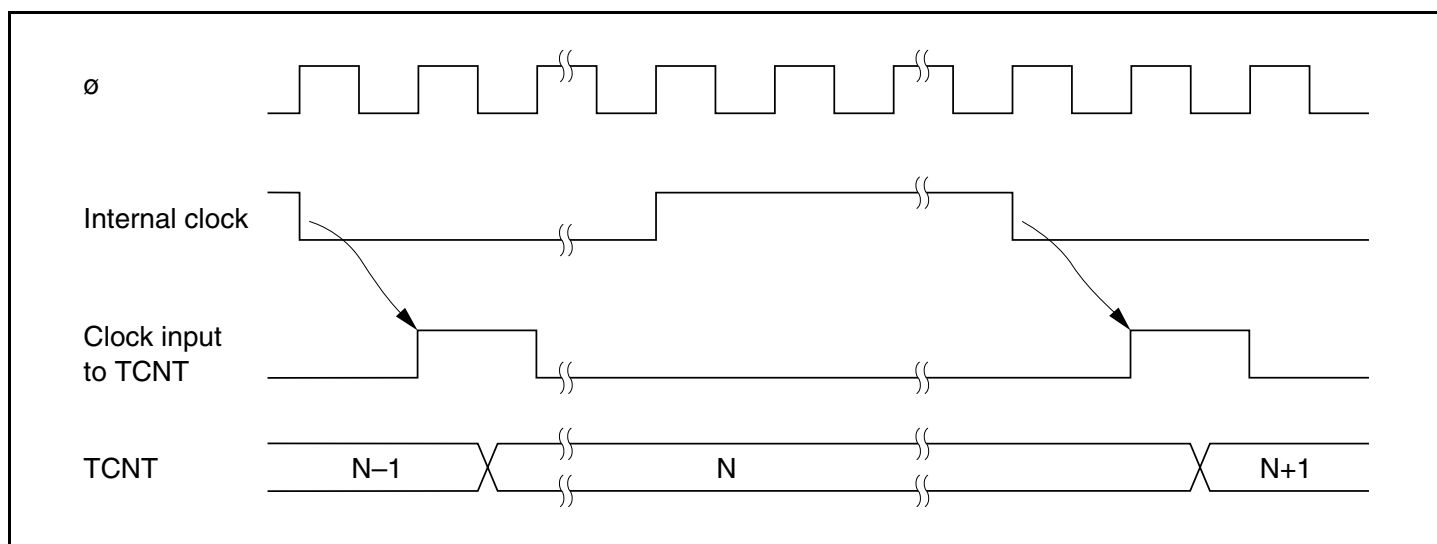
Figure 13.3 Count Timing for Internal Clock Input
