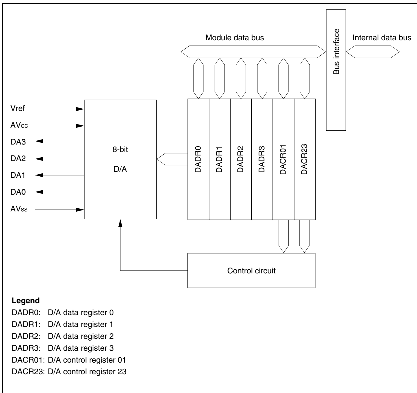
Figure 17.1 Block Diagram of D/A Converter
