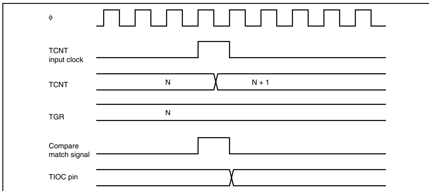
Figure 11.32 Output Compare Output Timing
