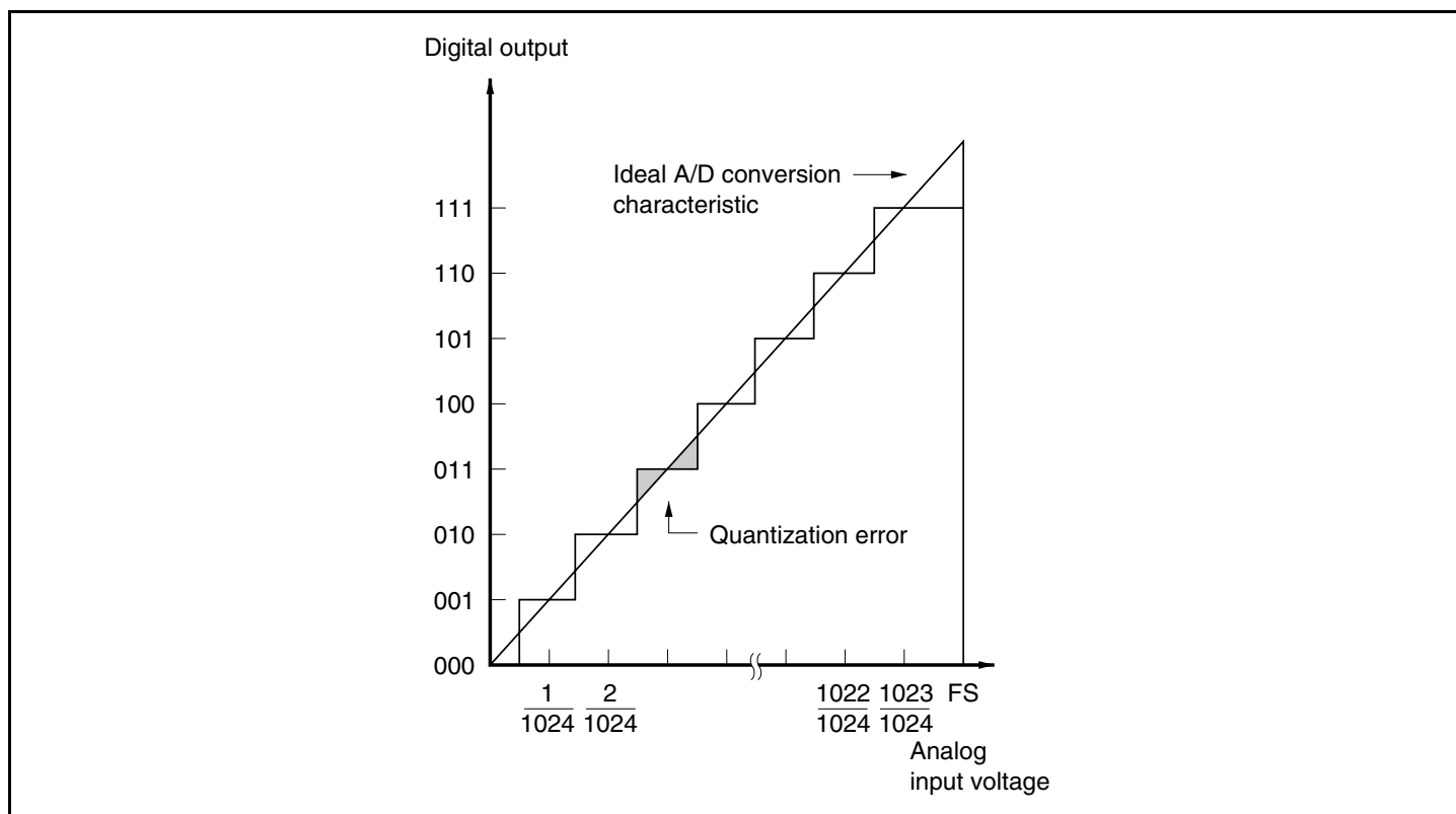
Figure 16.4 A/D Conversion Accuracy Definitions
