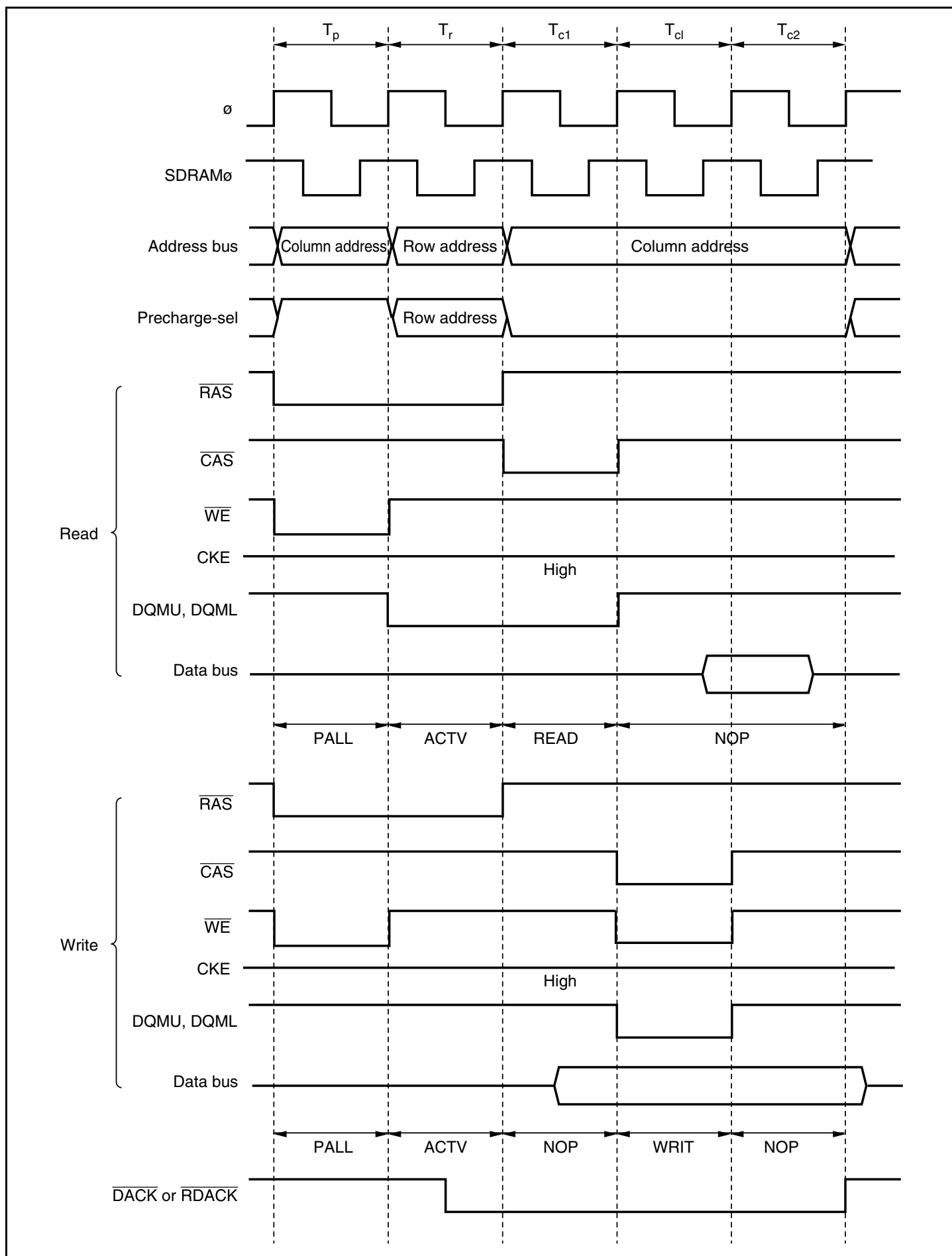
Figure 6.61 Example of DACK/EDACK Output Timing when DDS = 0 or EDDS = 0
