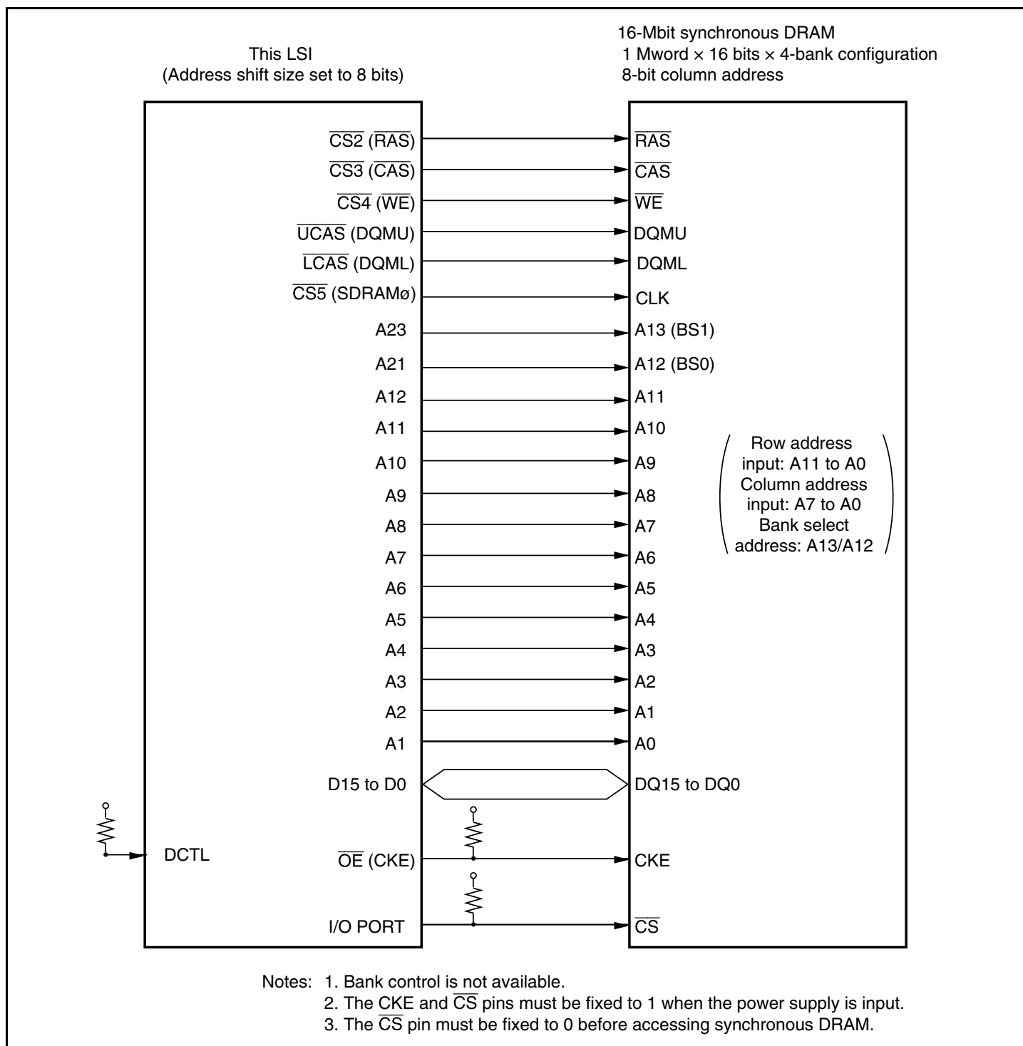
Figure 6.51 Example of DQMU and DQML Byte Control
