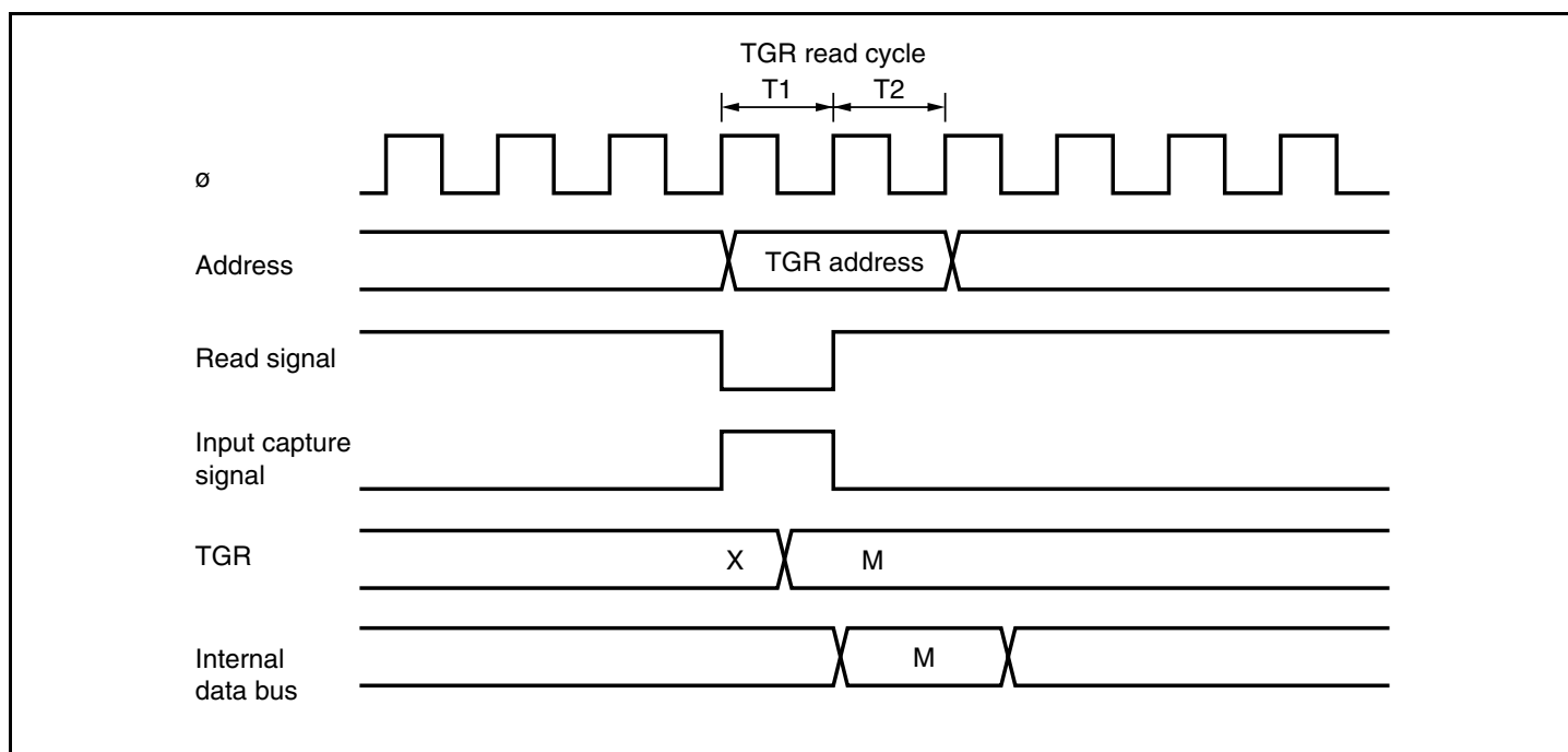
Figure 11.49 Contention between TGR Read and Input Capture
