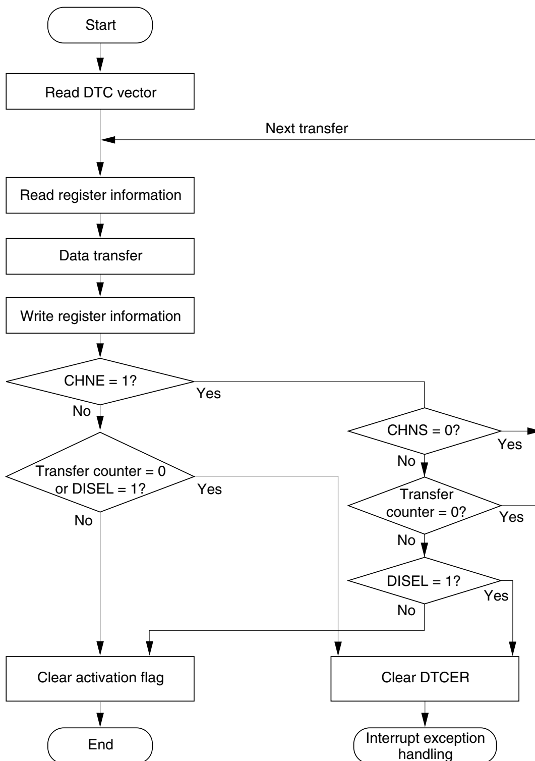
Figure 9.4 Flowchart of DTC Operation
