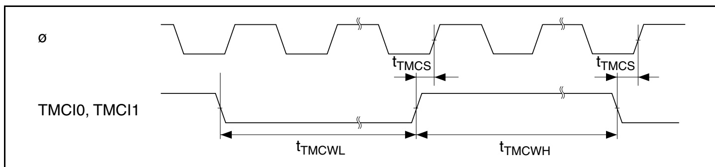
Figure 24.39 8-Bit Timer Clock Input Timing
