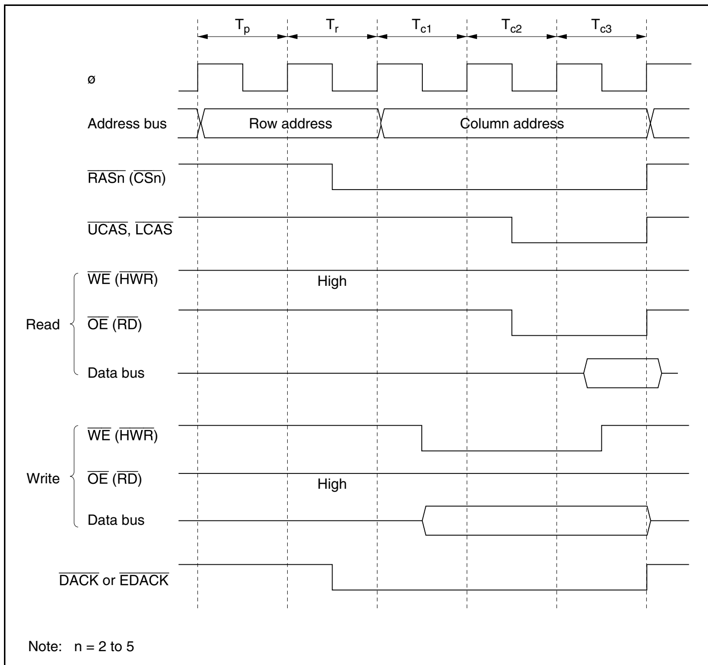
Figure 6.42 Example of DACK/EDACK Output Timing when DDS = 0 or EDDS = 0 (RAST = 0, CAST = 1)
