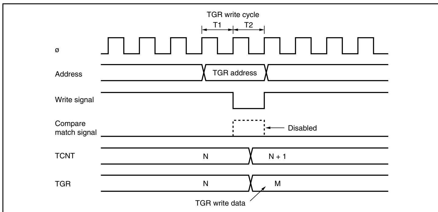
Figure 11.47 Contention between TGR Write and Compare Match
