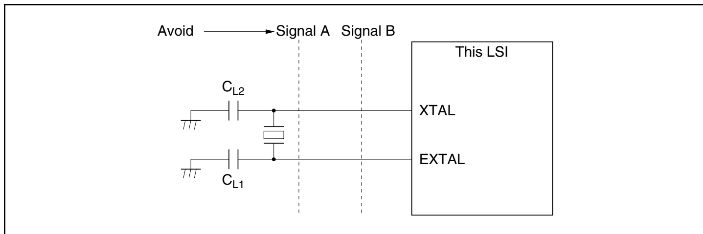
Figure 21.6 Note on Board Design for Oscillation Circuit
