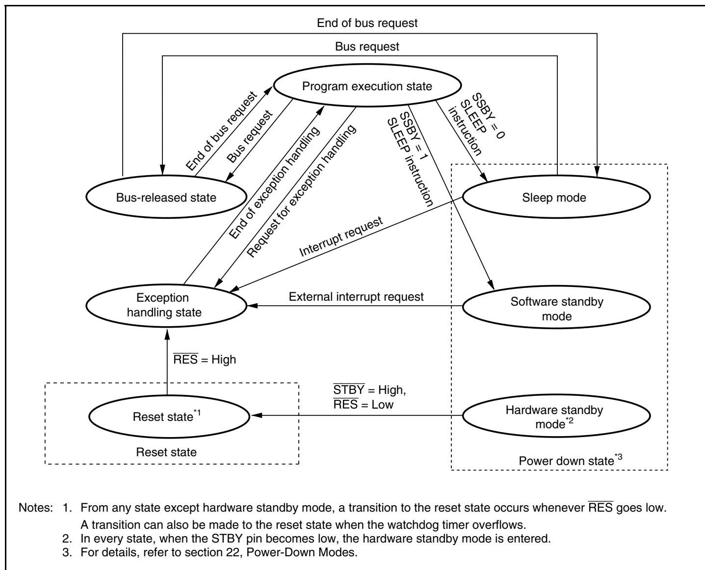
Figure 2.13 State Transitions
