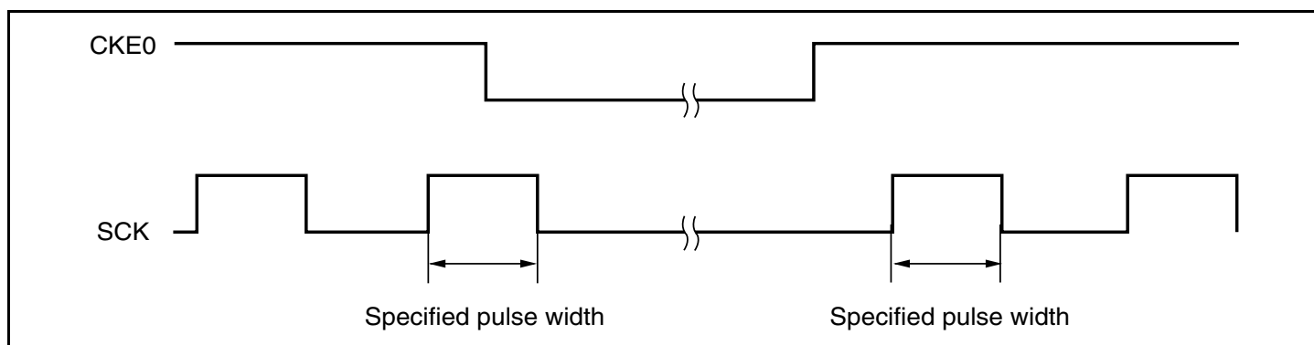
Figure 15.31 Timing for Fixing Clock Output Level
