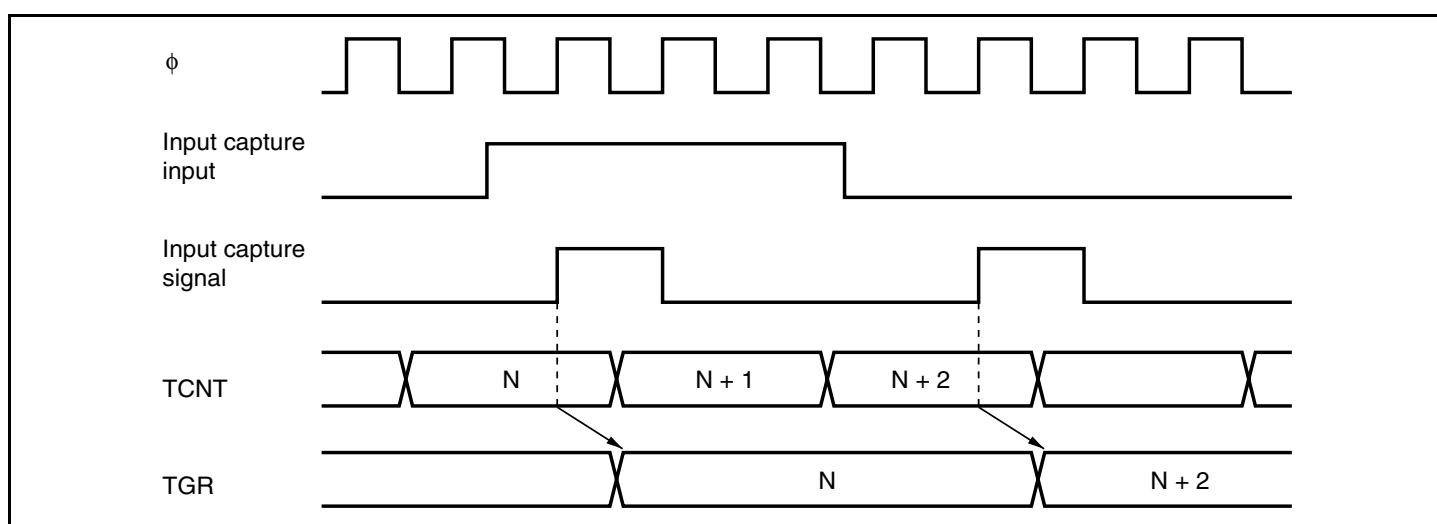
Figure 11.33 Input Capture Input Signal Timing
