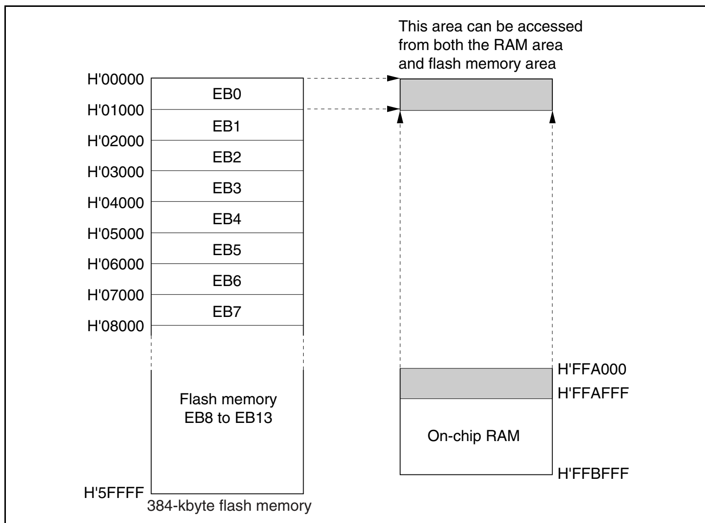
Figure 19.9 Example of RAM Overlap Operation
