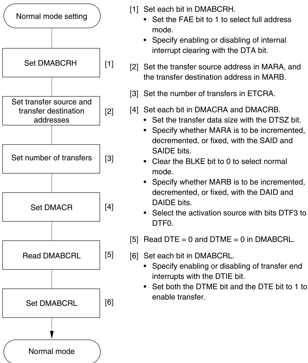
Figure 7.12 Example of Normal Mode Setting Procedure
