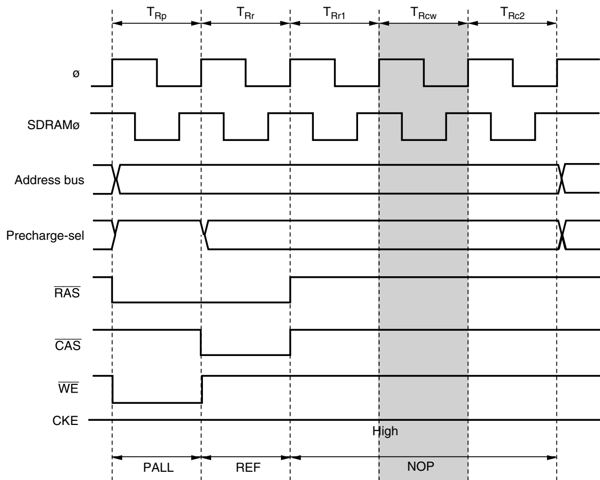
Figure 6.56 Auto Refresh Timing (TPC = 0, TPC0 = 0, RLW1 = 0, RLW0 = 1)
