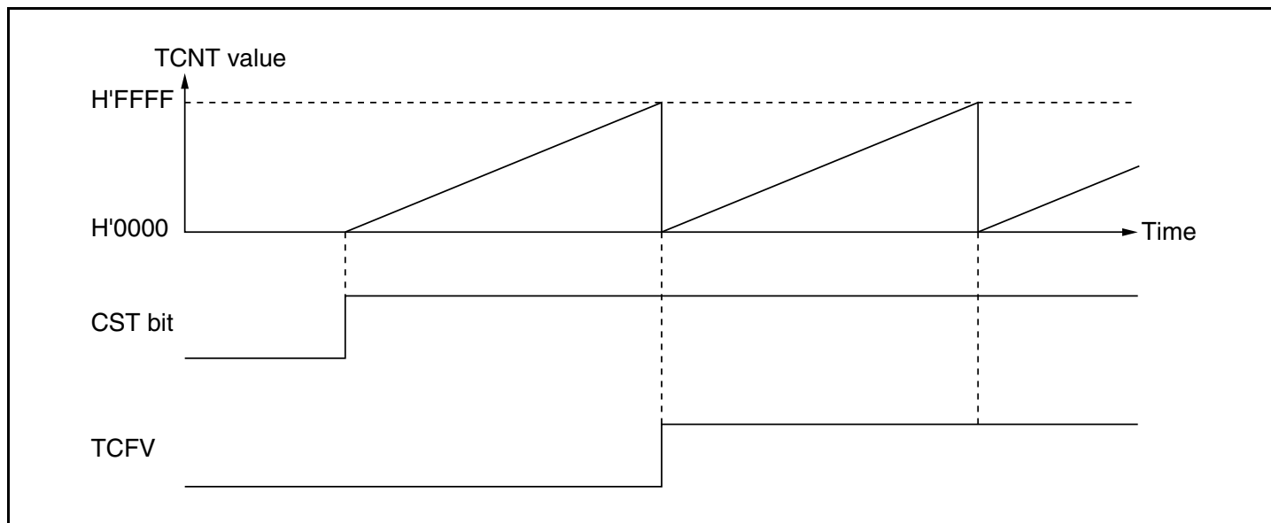
Figure 11.3 Free-Running Counter Operation
