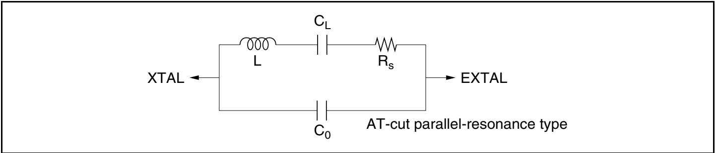
Figure 21.3 Crystal Resonator Equivalent Circuit
