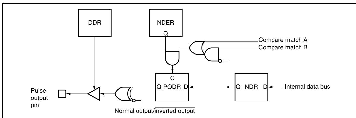
Figure 12.6 Non-Overlapping Pulse Output
