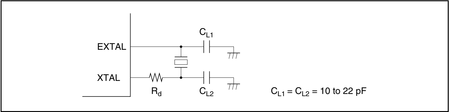
Figure 21.2 Connection of Crystal Resonator (Example)
