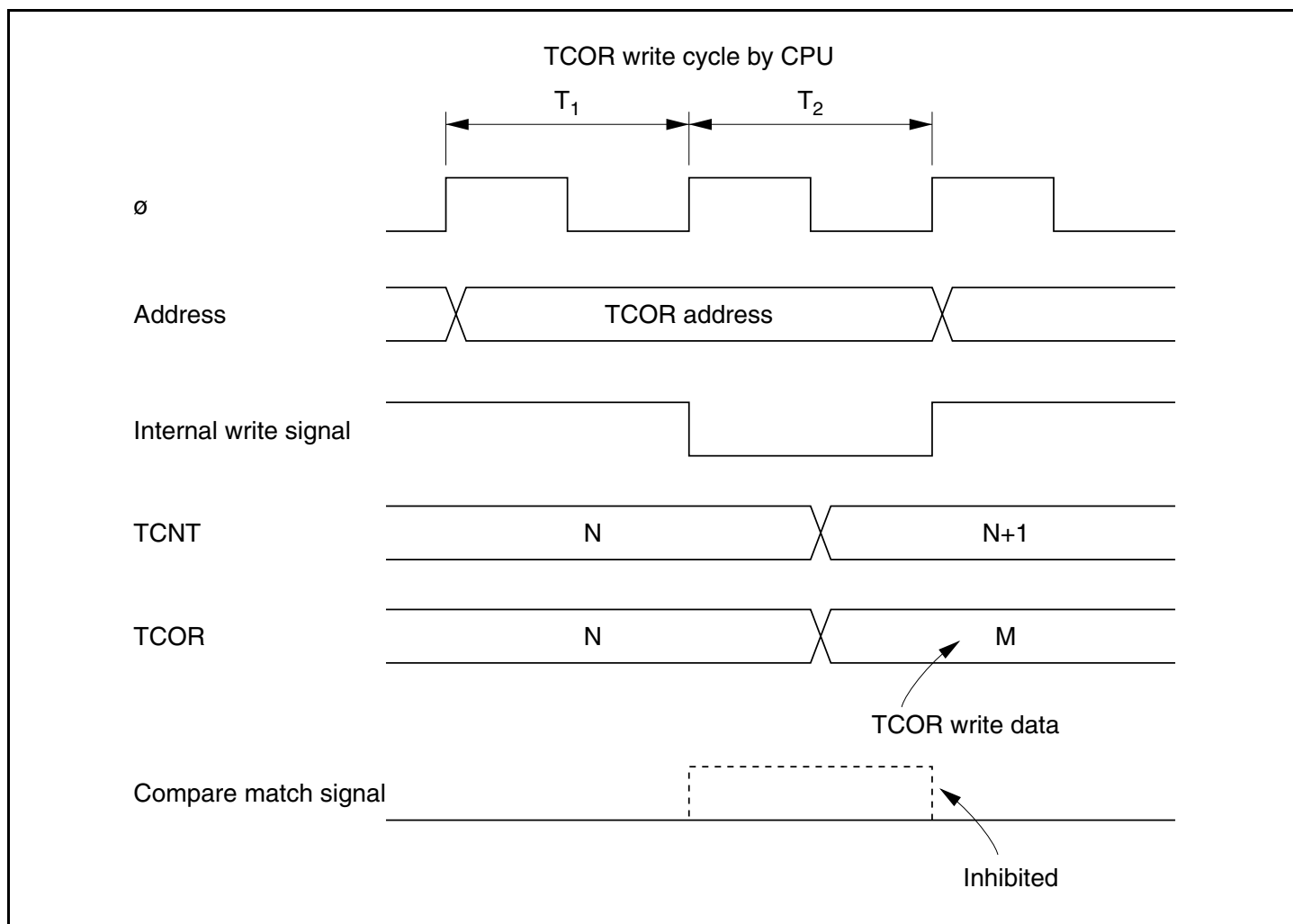
Figure 13.12 Contention between TCOR Write and Compare Match
