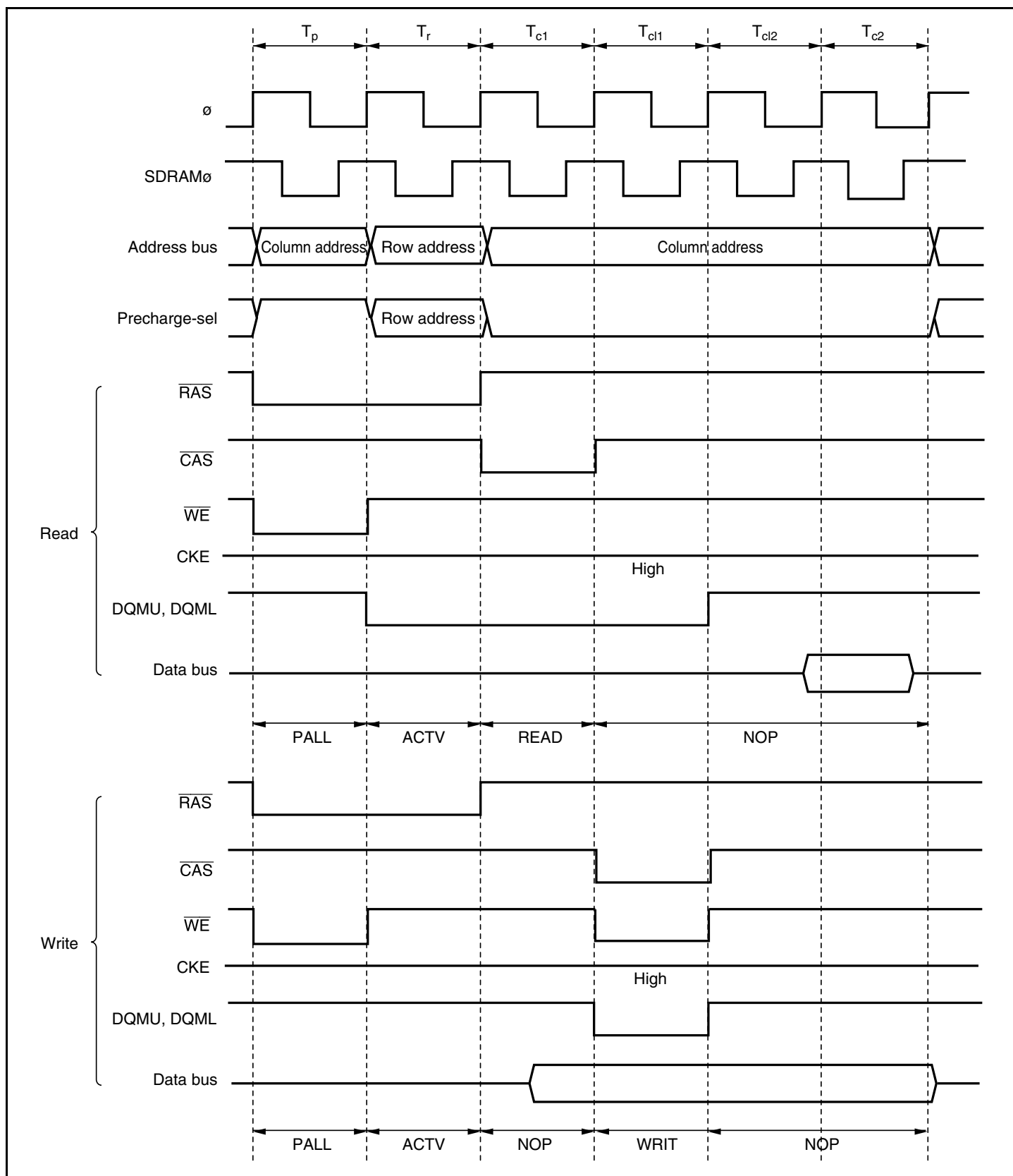
Figure 6.45 CAS Latency Control Timing (SDWCD = 0, CAS Latency 3)
