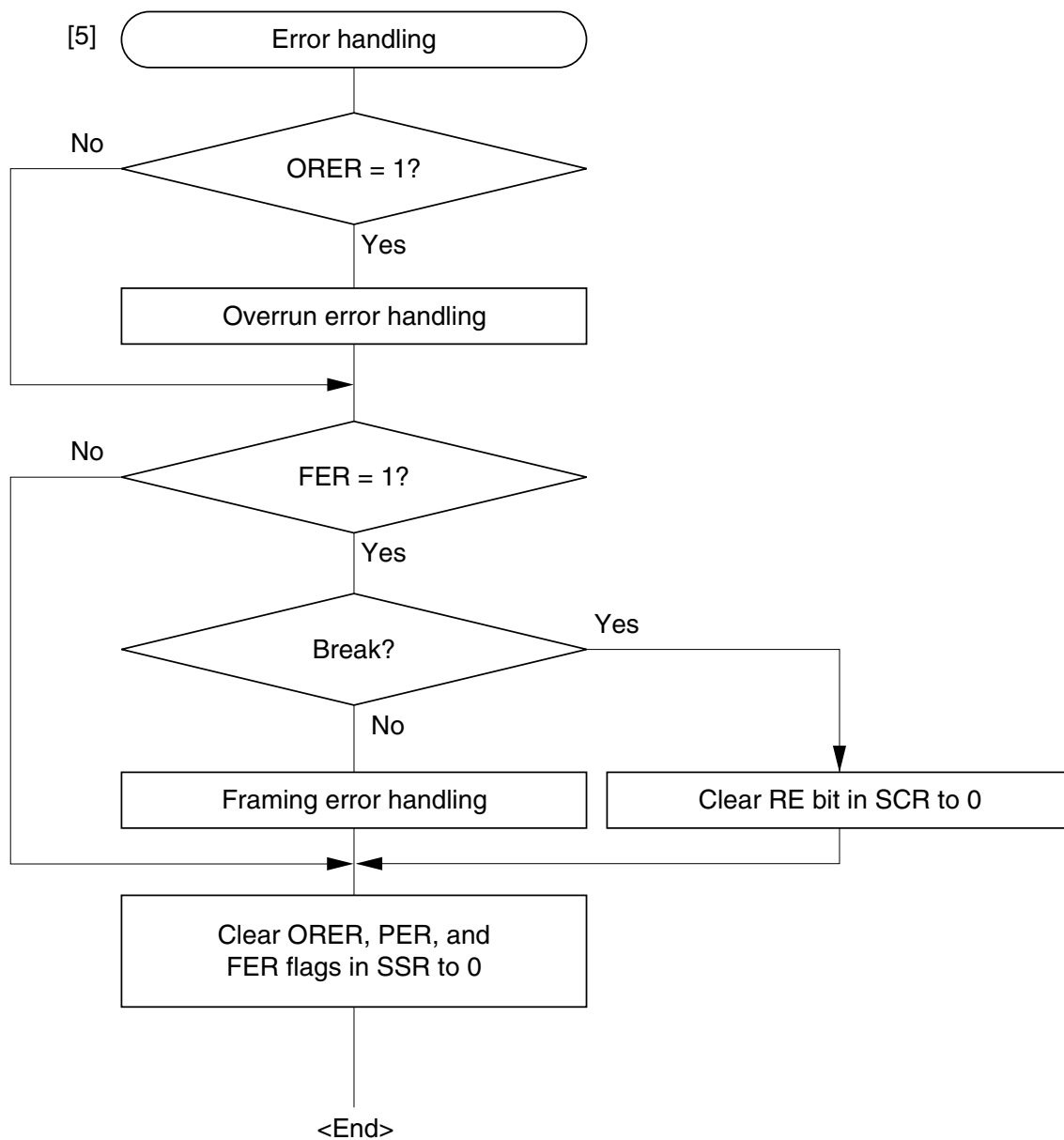
Figure 15.13 Sample Multiprocessor Serial Reception Flowchart (2)
