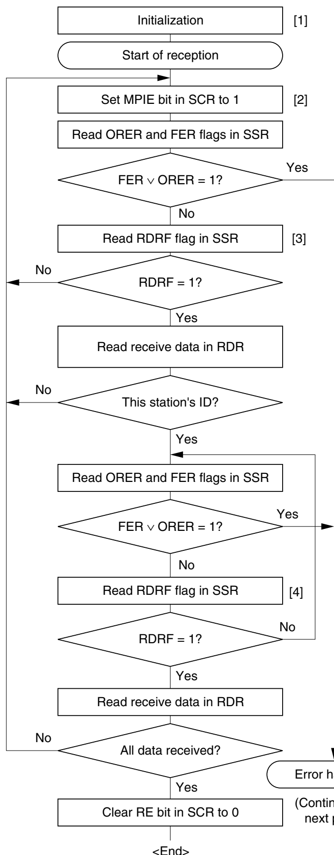
Figure 15.13 Sample Multiprocessor Serial Reception Flowchart (1)
