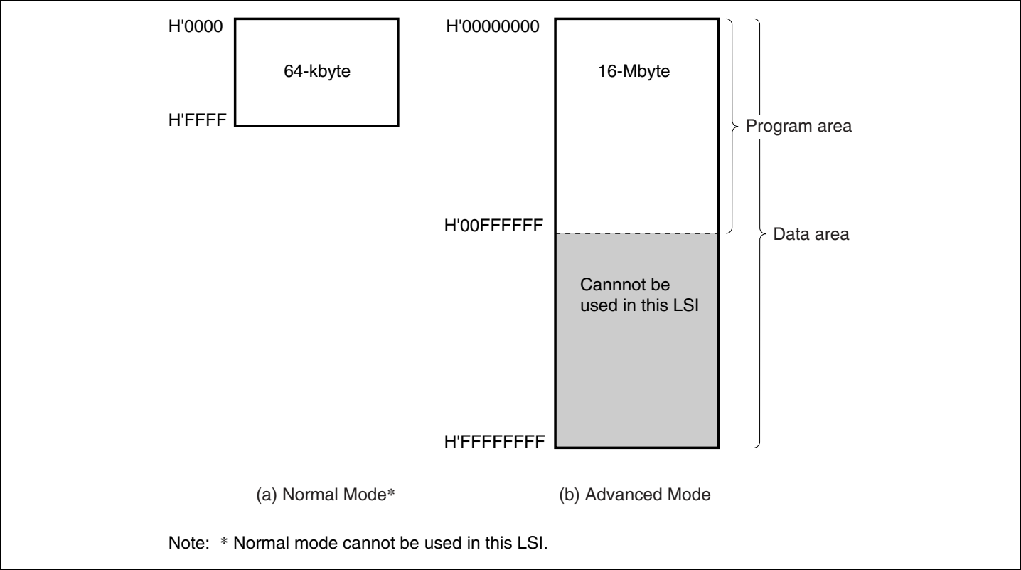
Figure 2.5 Memory Map
