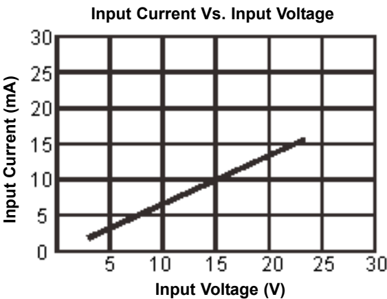
Characteristic Curves
