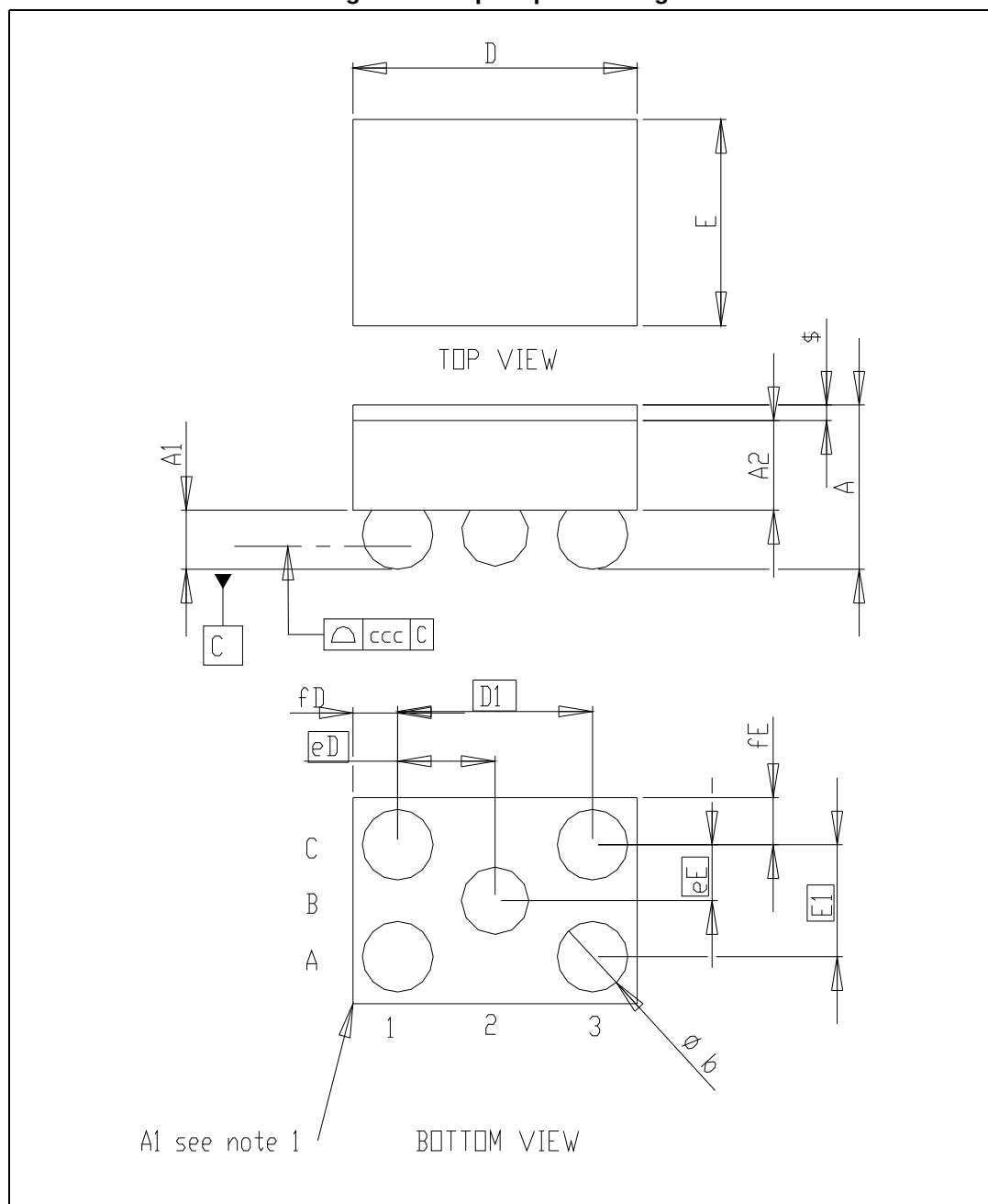
Figure 23. Flip-chip 5 drawings
