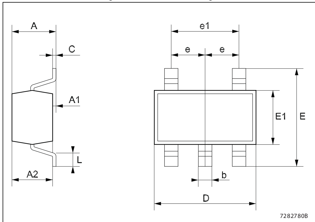
Figure 26. TSOT23-5L drawings
