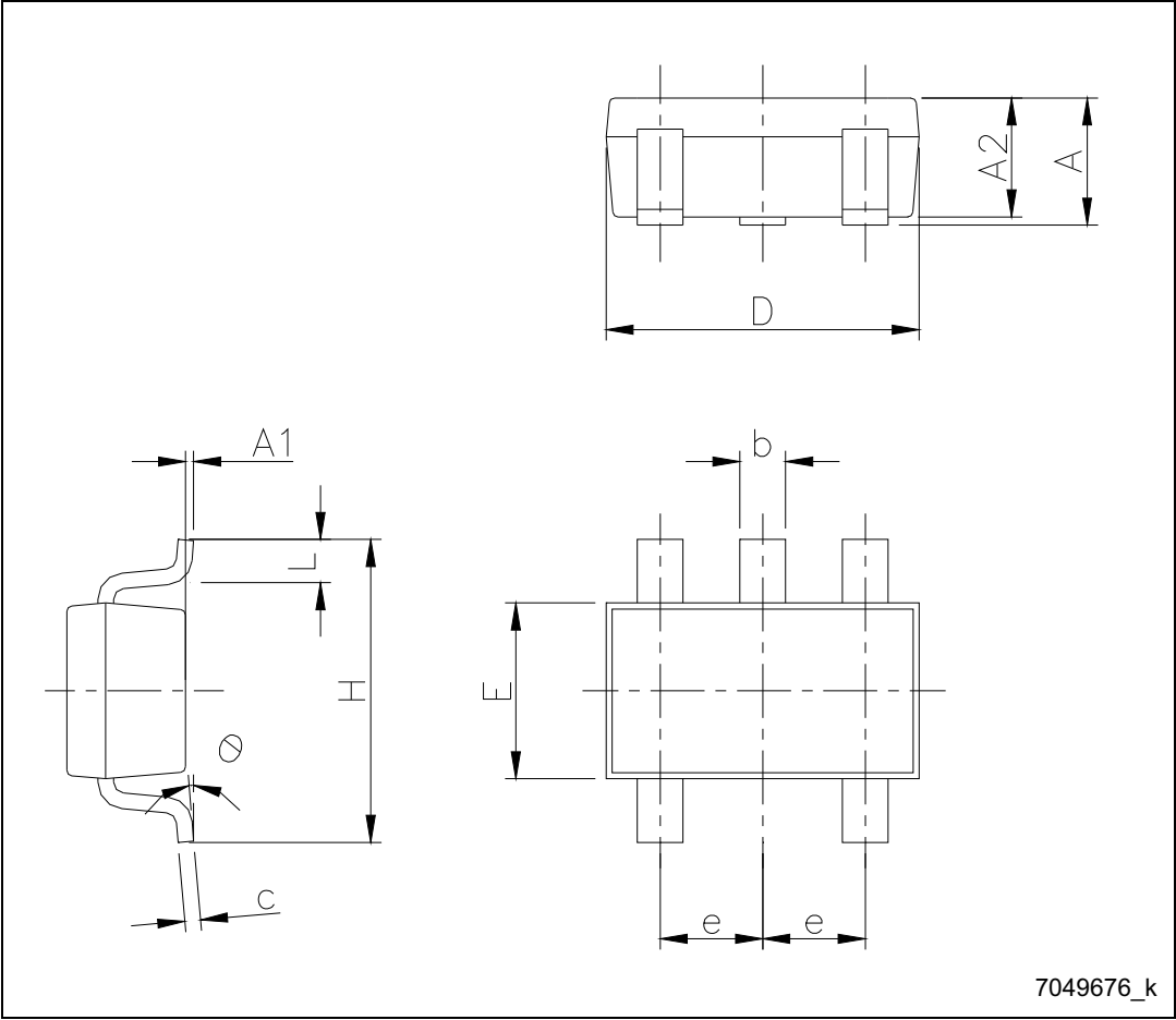
Figure 24. SOT23-5L drawings
