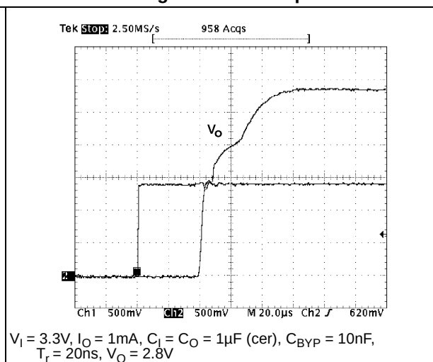
Figure 21. Start-up
