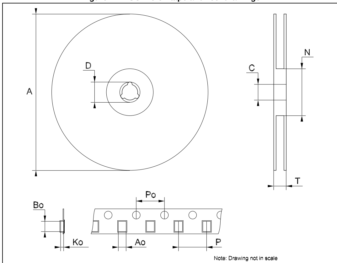
Figure 27. TSOT23-5L tape and reel drawings
