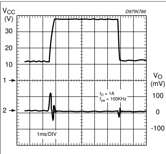
Figure 22. Line transient
