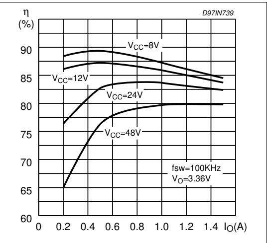
Figure 15. Efficiency vs. output current
