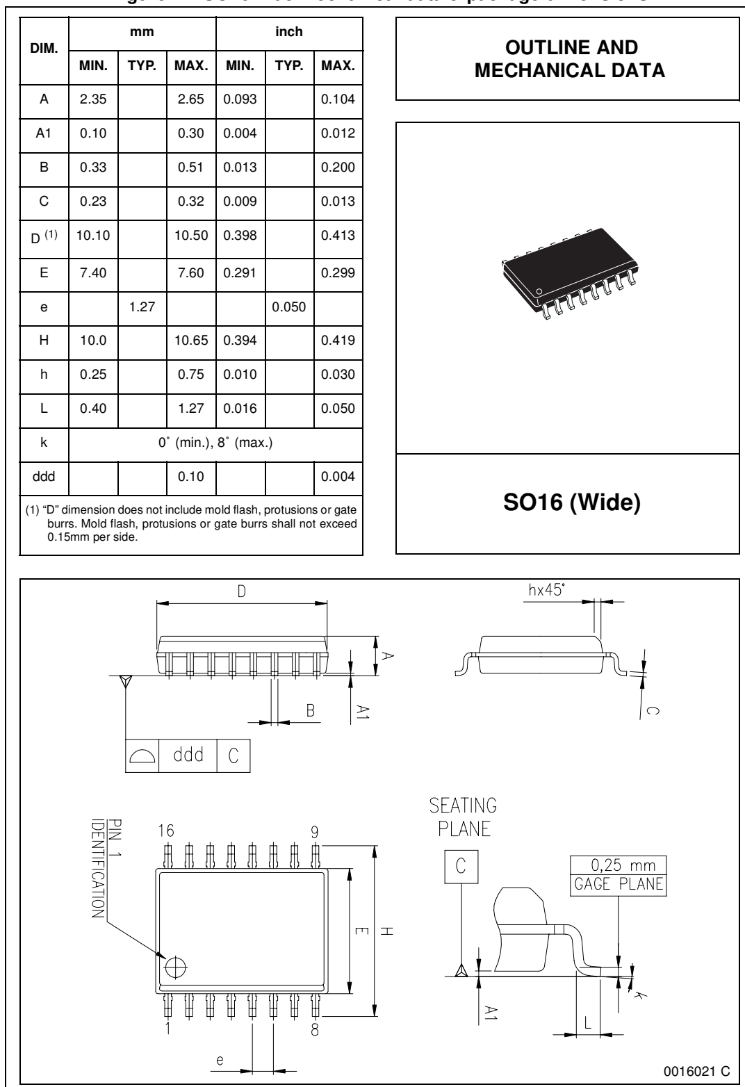
Figure 24. SO16Wide mechanical data &amp; package dimensions
