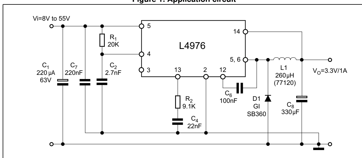
Figure 1. Application circuit
