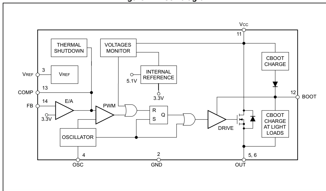
Figure 2. Block diagram
