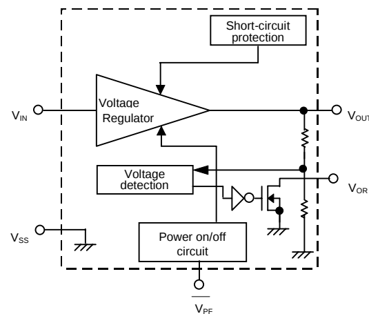
Figure 2 Block Diagram
