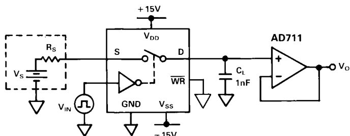
Test Circuit 5. Charge Injection
