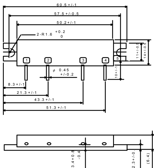
OUTLINE DRAWING
