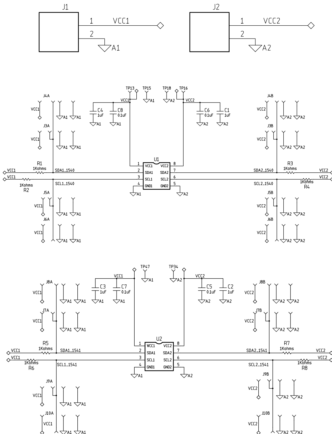
Figure 1-3. ISO154xEVM Schematic
