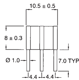
2) 4.4 Leg Pitch = R SL1024A xxxR
