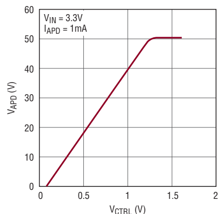
APD Voltage Adjustment with CTRL
