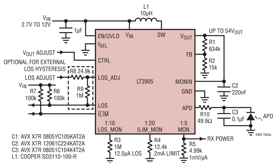
Low Noise APD Bias with External LOS Threshold
