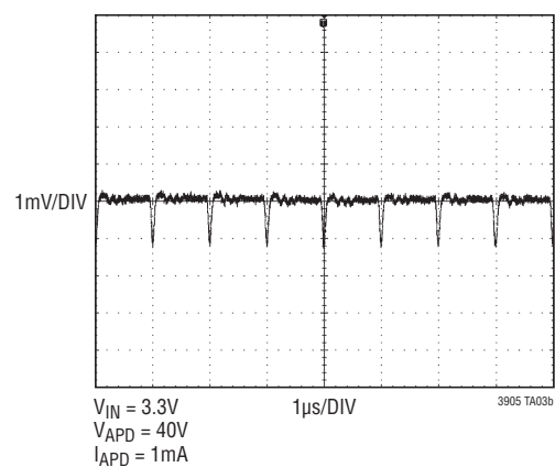
APD Bias Ripple
