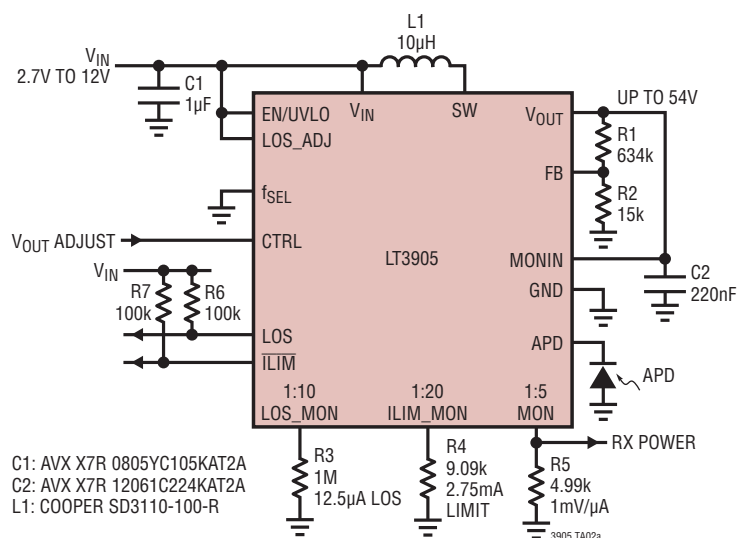
Adjustable APD Bias Supply
