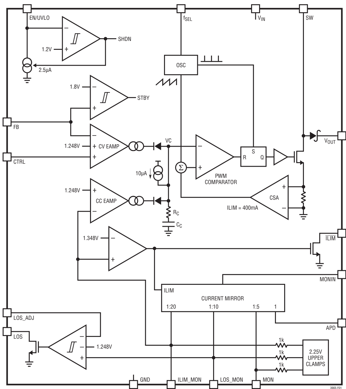
Figure 1. Block Diagram
