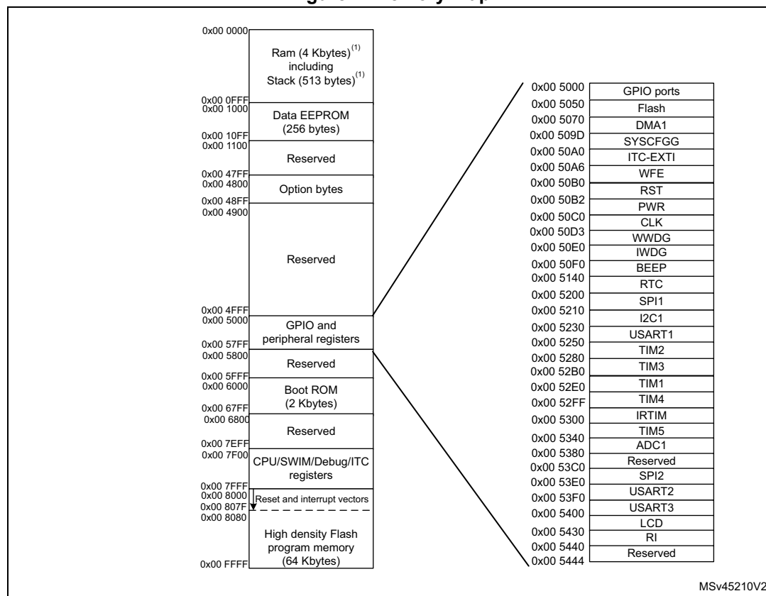
Figure 4. Memory map
