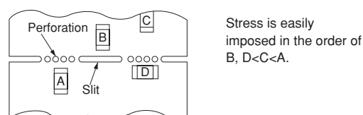
[Chip Mounting Close to Board Separation Point]
