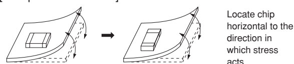
[Chip Mounting Close to Board Separation Point]
