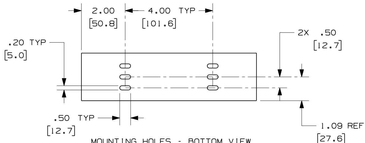
MOUNTING HOLES - BOTTOM VIEW HS2X2**2 AND HS2X2**6 ONLY
