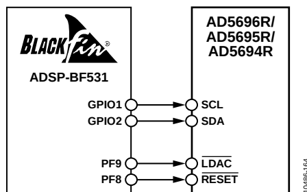
Figure 56. ADSP-BF531 Interface
