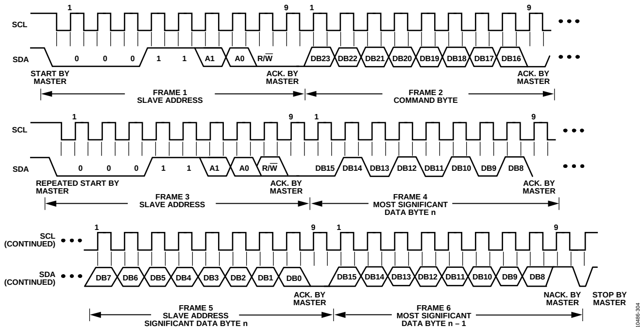
Figure 51. I²C Read Operation
