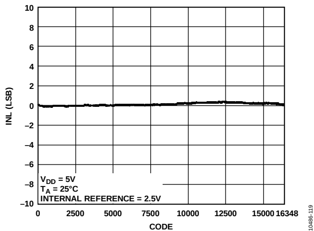
Figure 13. AD5695R INL
