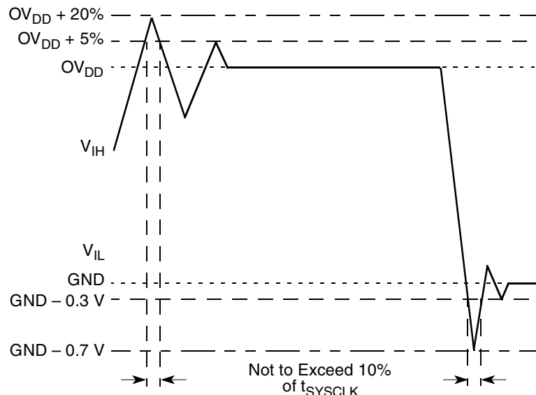
Figure 2. Overshoot/Undershoot Voltage
