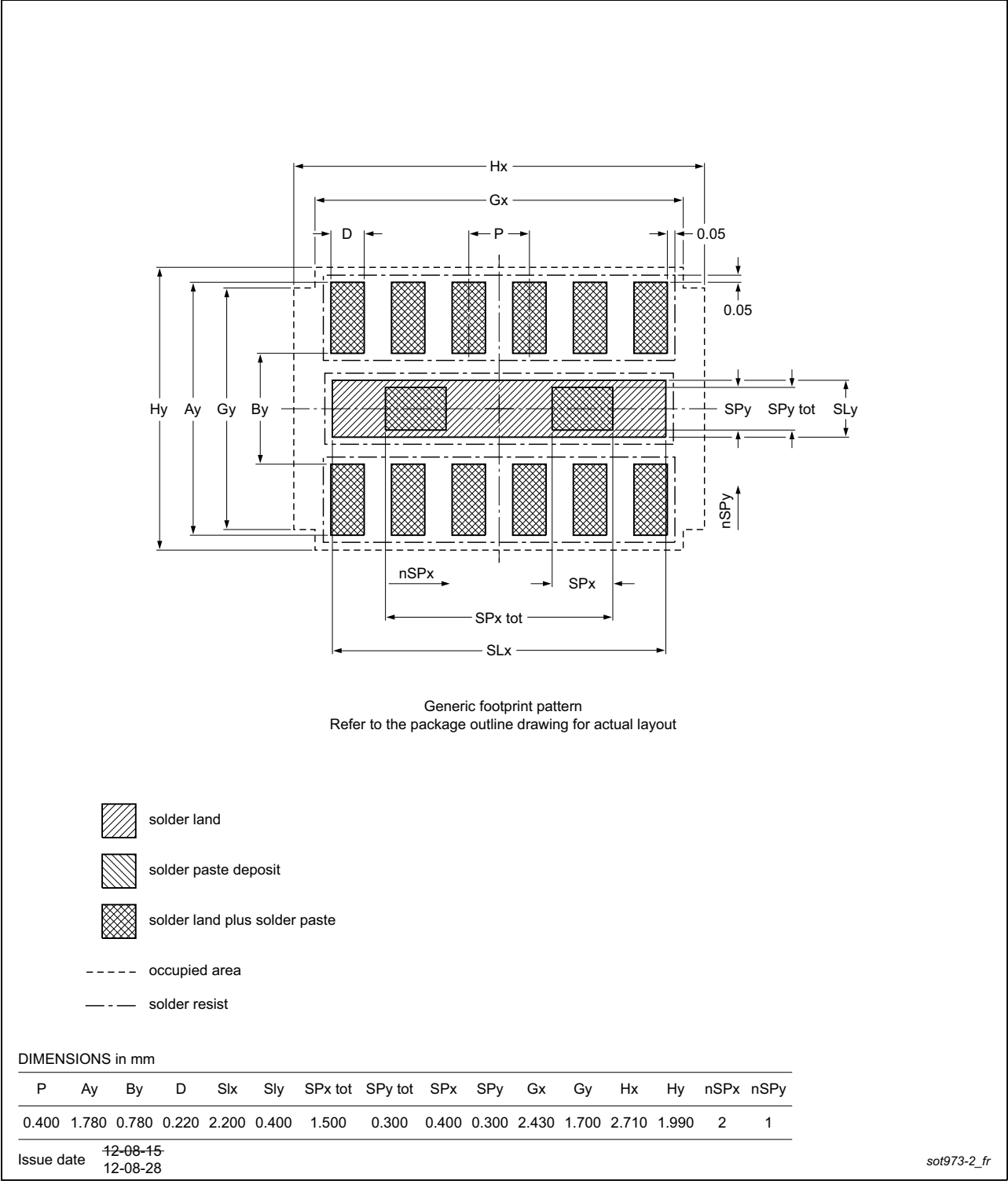
Fig 24. PCB footprint for SOT973-2 (HXSON12); reflow soldering
