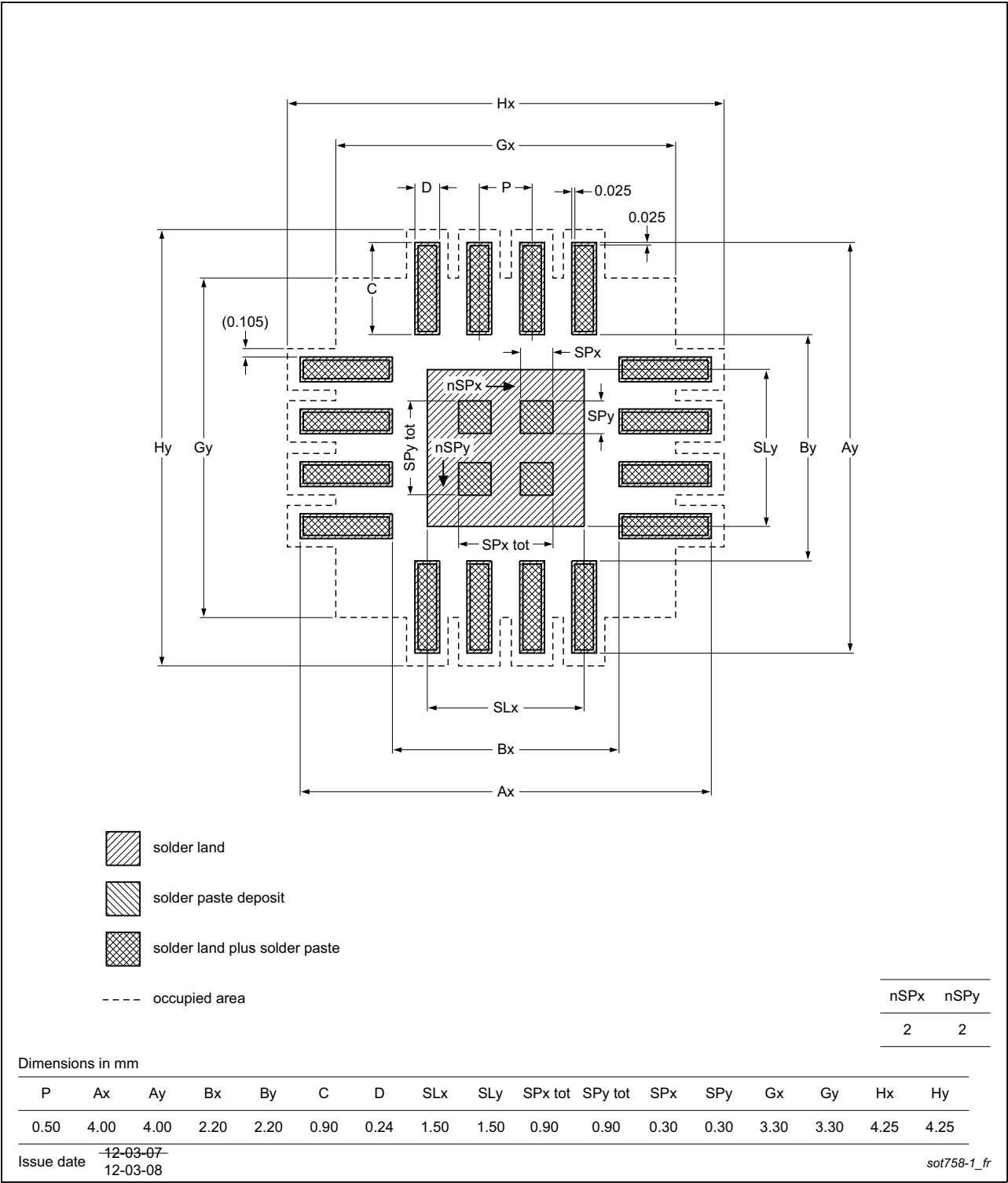
Footprint information for reflow soldering of HVQFN16 package SOT758-1
