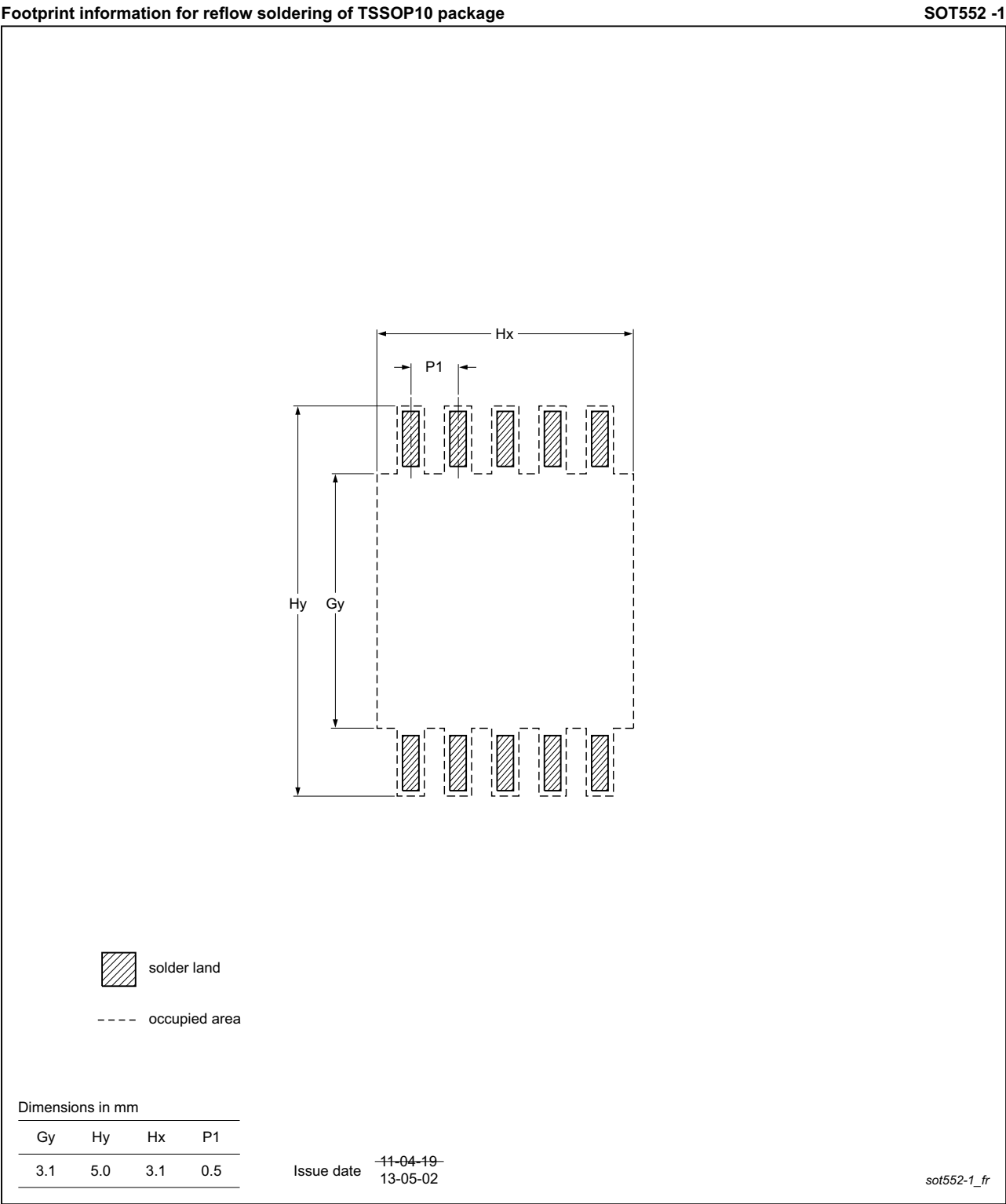
Fig 23. PCB footprint for SOT552-1 (TSSOP10); reflow soldering
